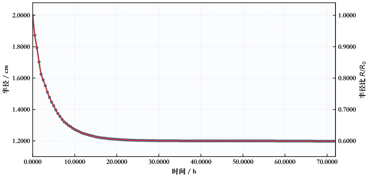
附件2半径实测点与PCHIP插值及半径比
