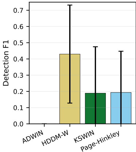
Faces
