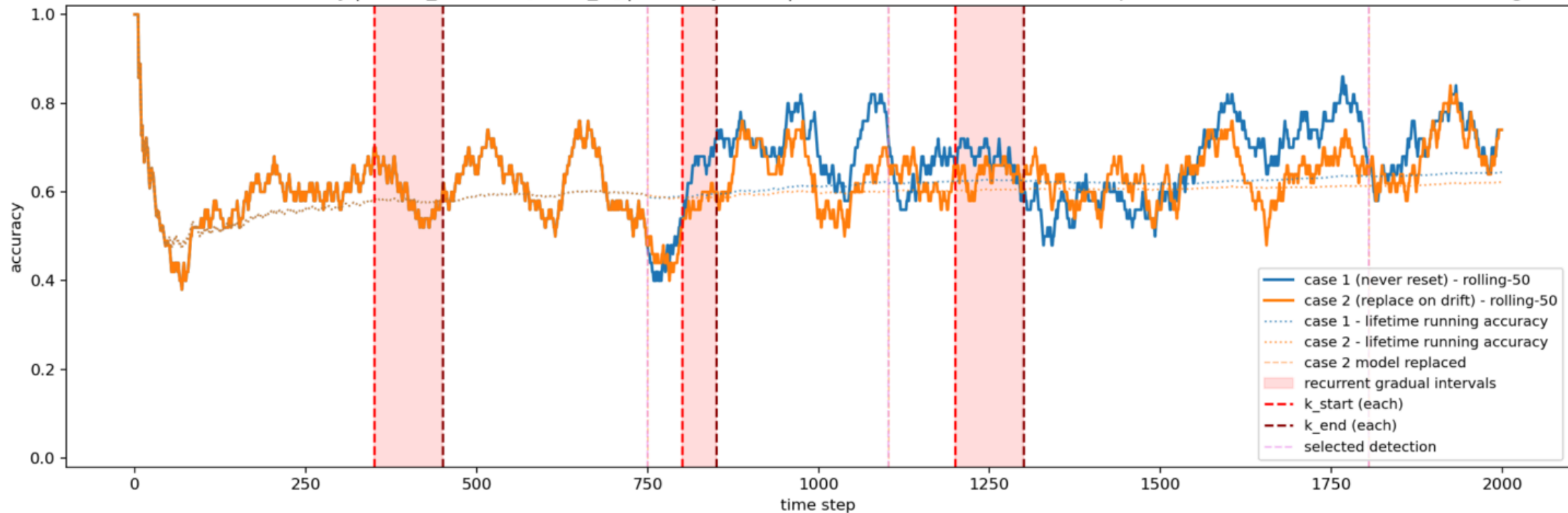
Online classifier accuracy | HDDM_W (river) [hddm_w] | modality=both | case 1 = never reset, case 2 = replace on drift (shadow starts after warning)
