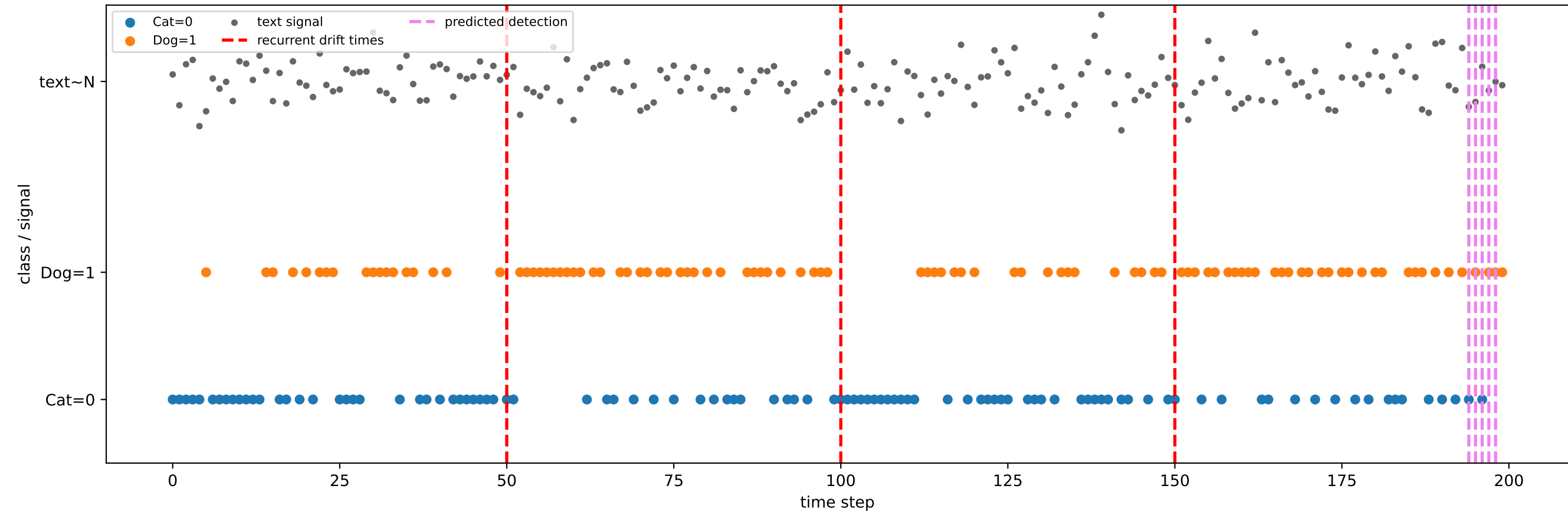
Semi-synthetic multimodal stream with recurrent drift
