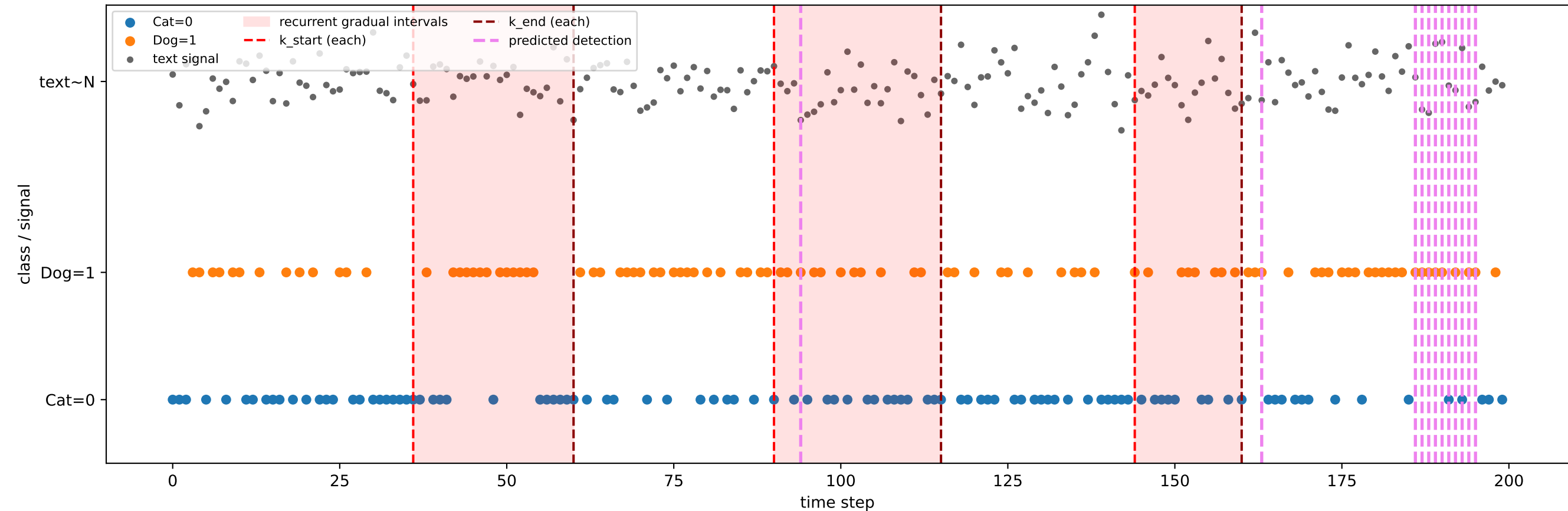
Semi-synthetic multimodal stream with recurrent gradual drift
