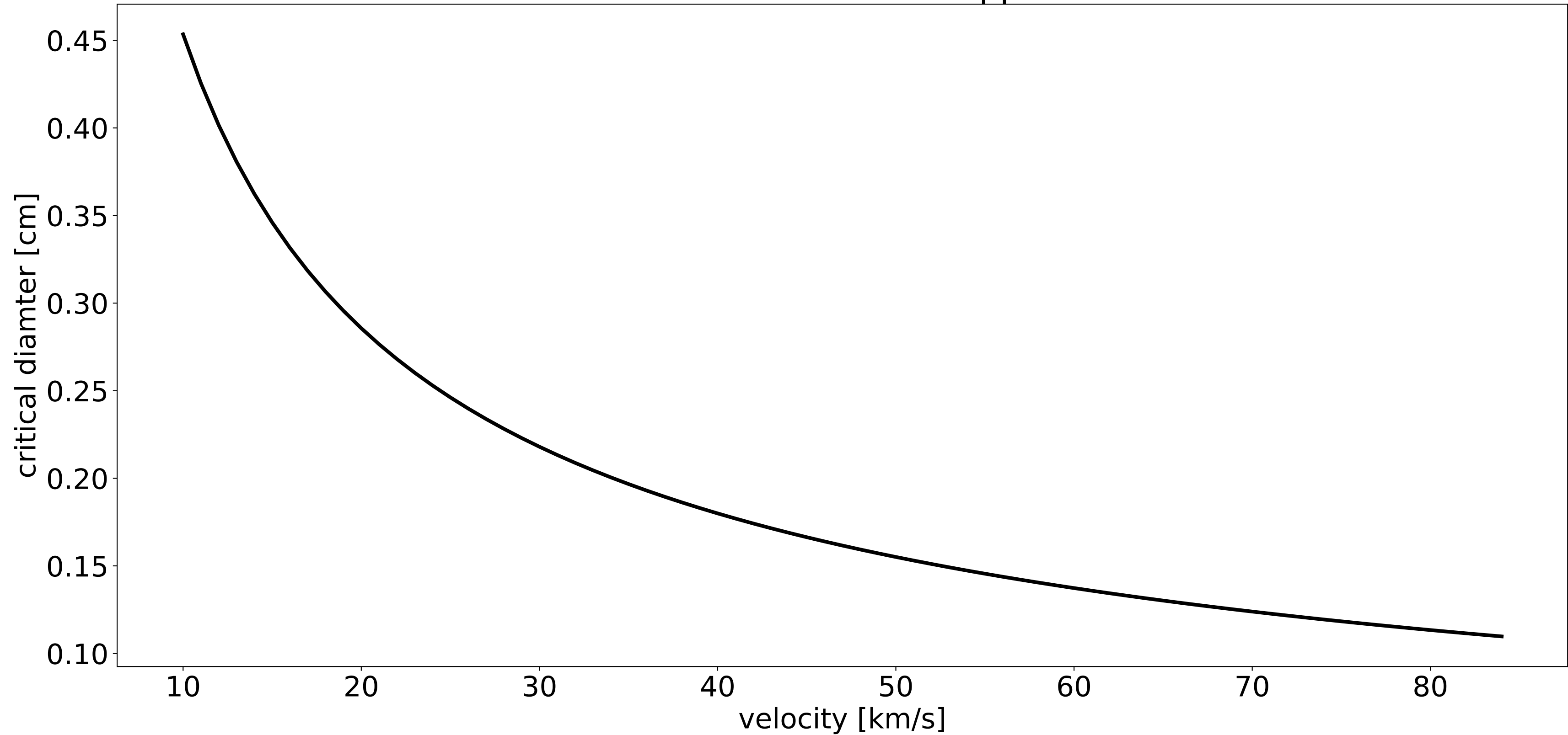
Ballistic Limit Curve for Whipple Shield
