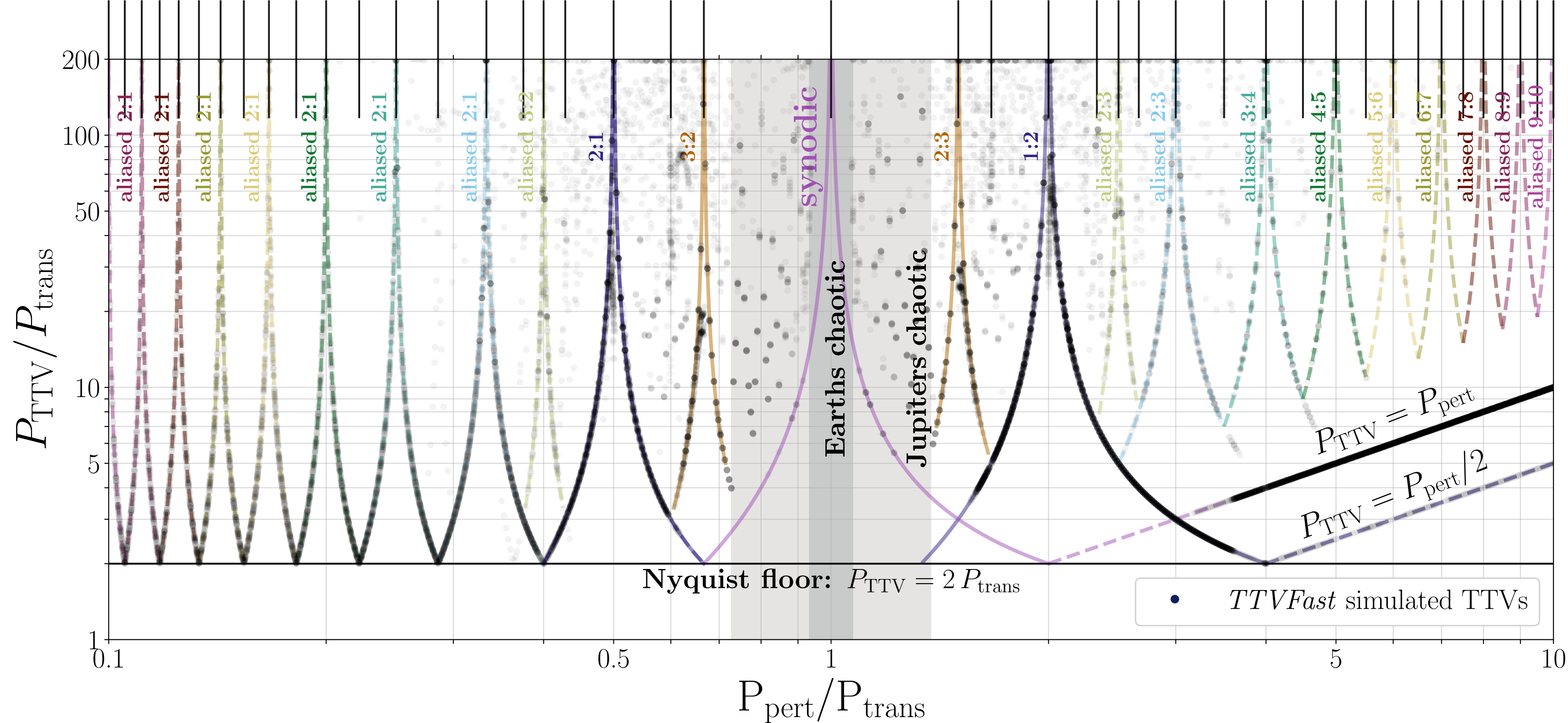
suggested priors on orbital period ratio based on multi-modalities
