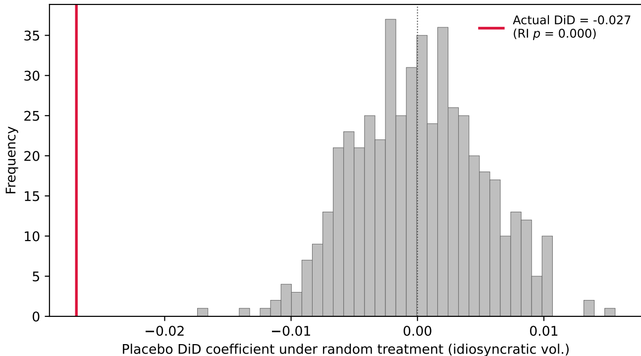
Randomization inference: 500 permutations of treatment
