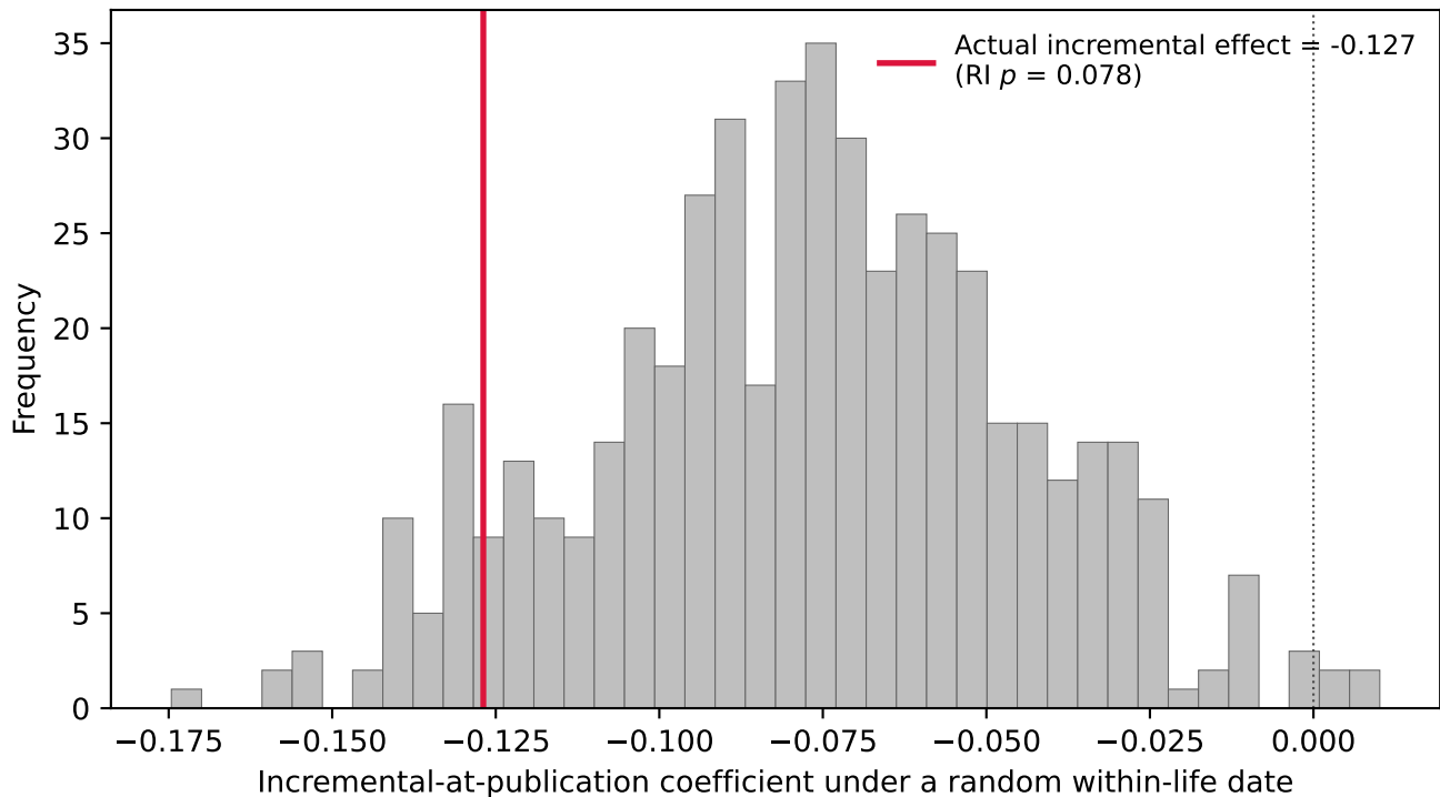
Timing-specificity test: is the drop tied to the TRUE publication date?
