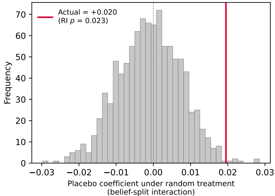
Belief-split interaction
