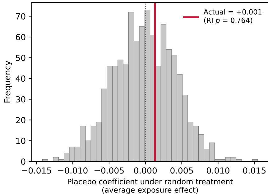
Average exposure effect
