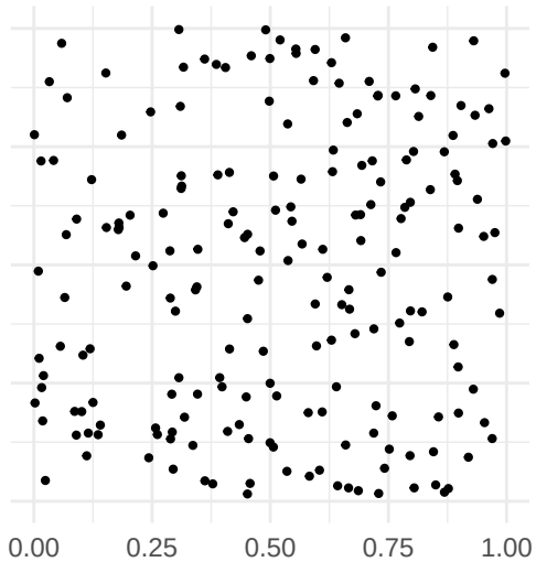
Pseudo-random
