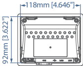
Rear View
