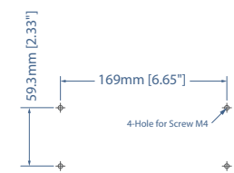
Screw Hole Dimensions
