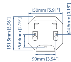
Mounting Brackets
