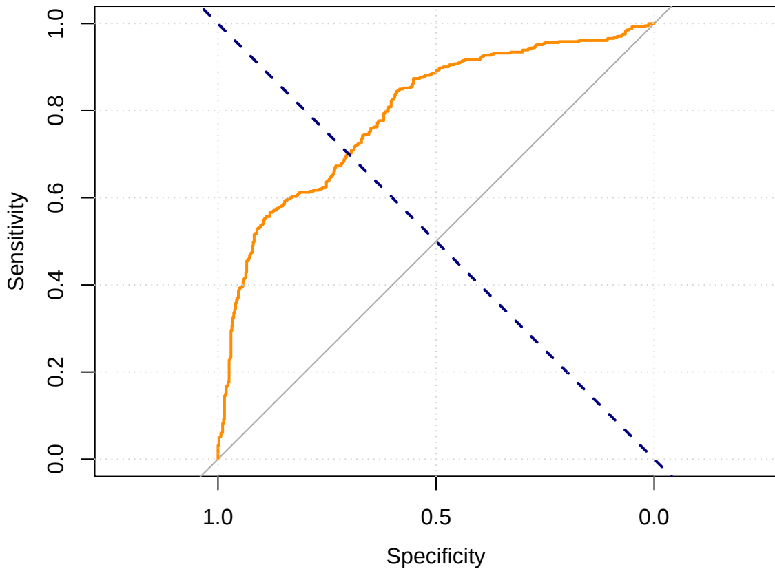
ROC Curve – High Admission (AUC = 0.793)
