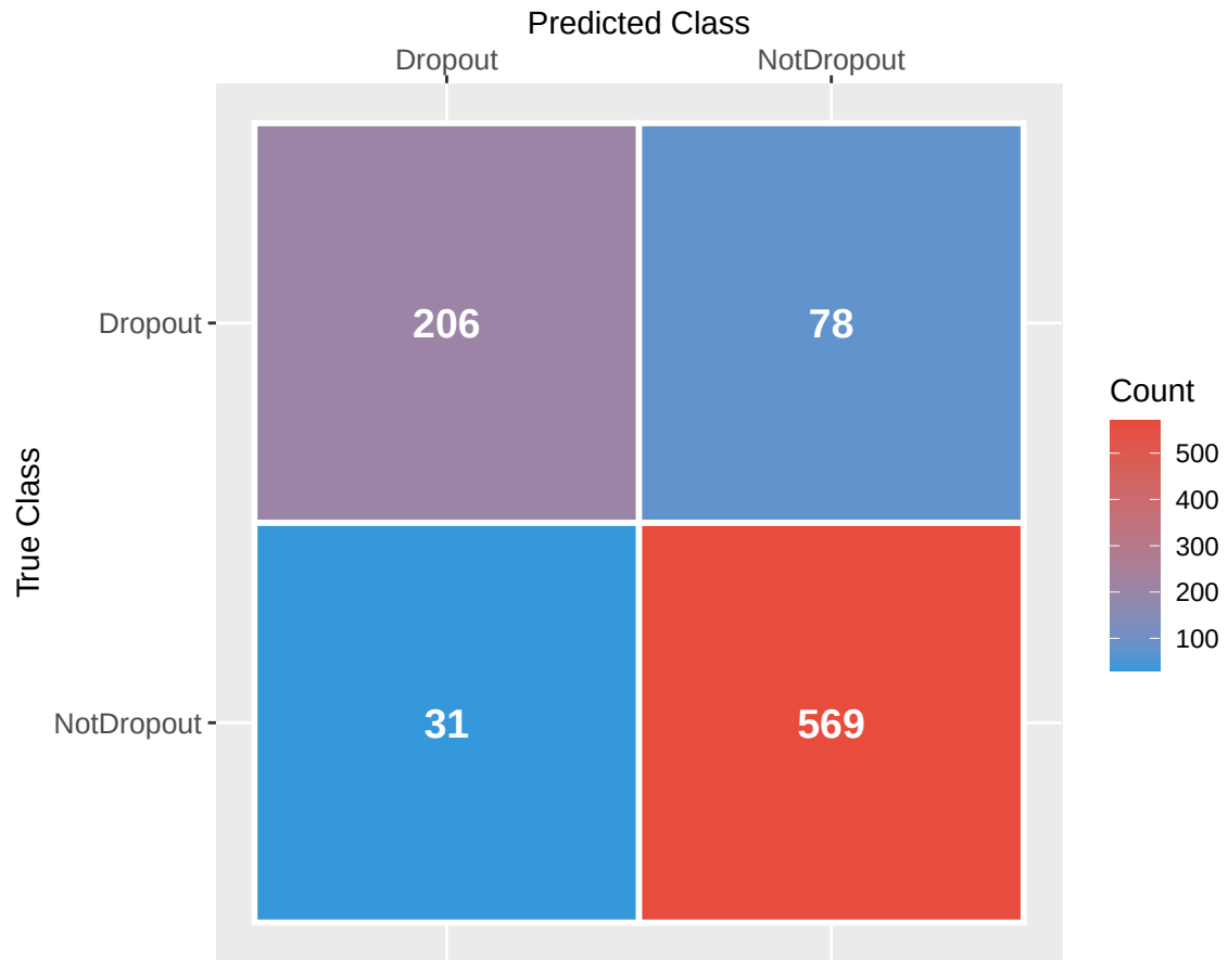
Model B: neuralnet (3 hidden layers)
