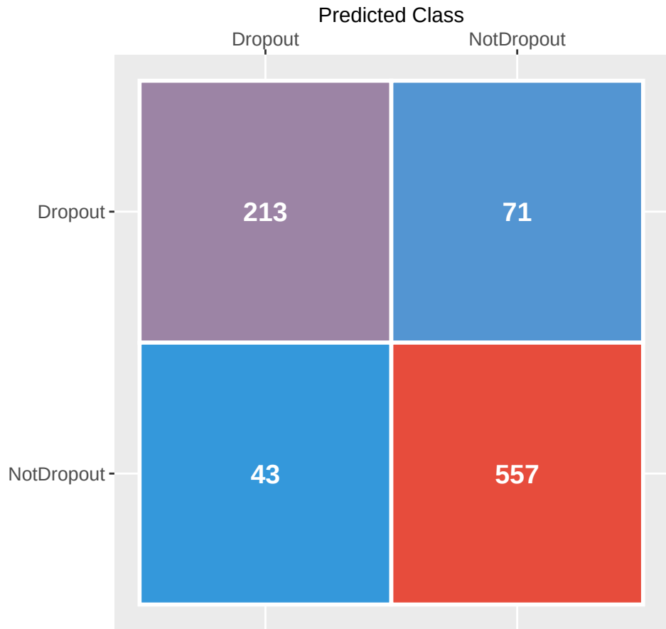
Model A: nnet (1 hidden layer)
