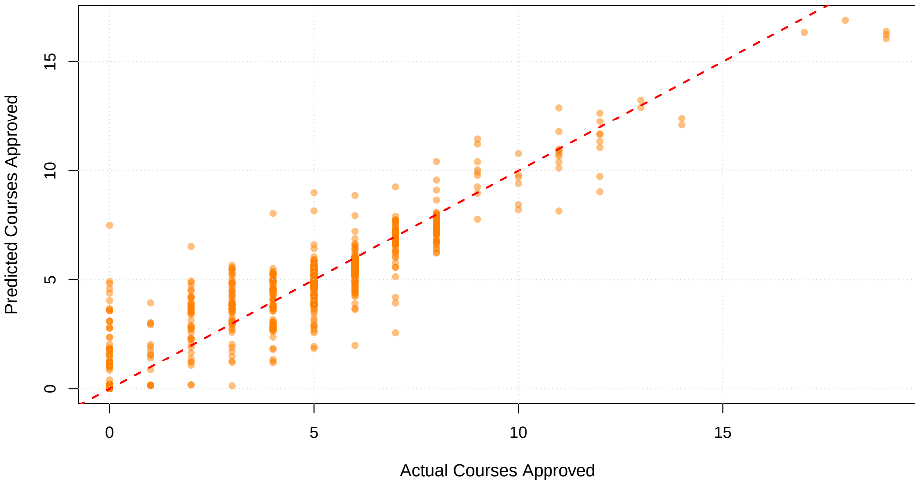
Poisson GAM ( R^2 = 0.8606 )
