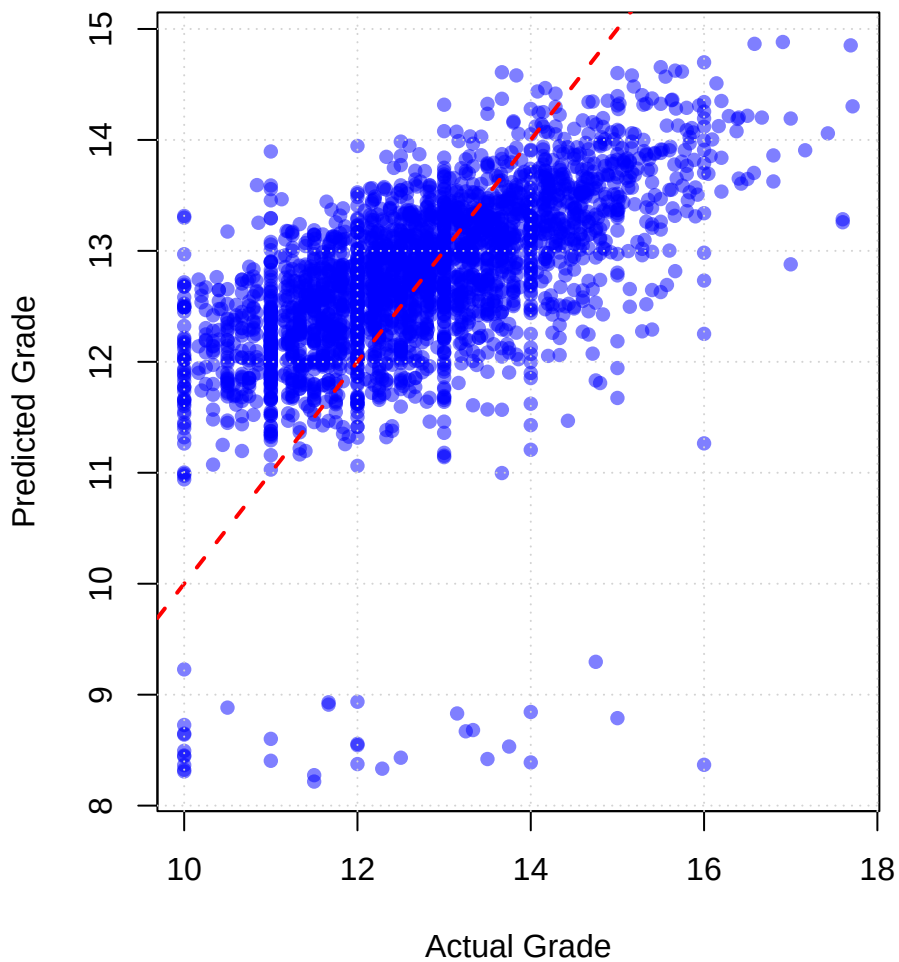
Training Set ( R^2 = 0.3302 )
