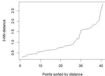
3-NN distance plot (CP1, CP2)
