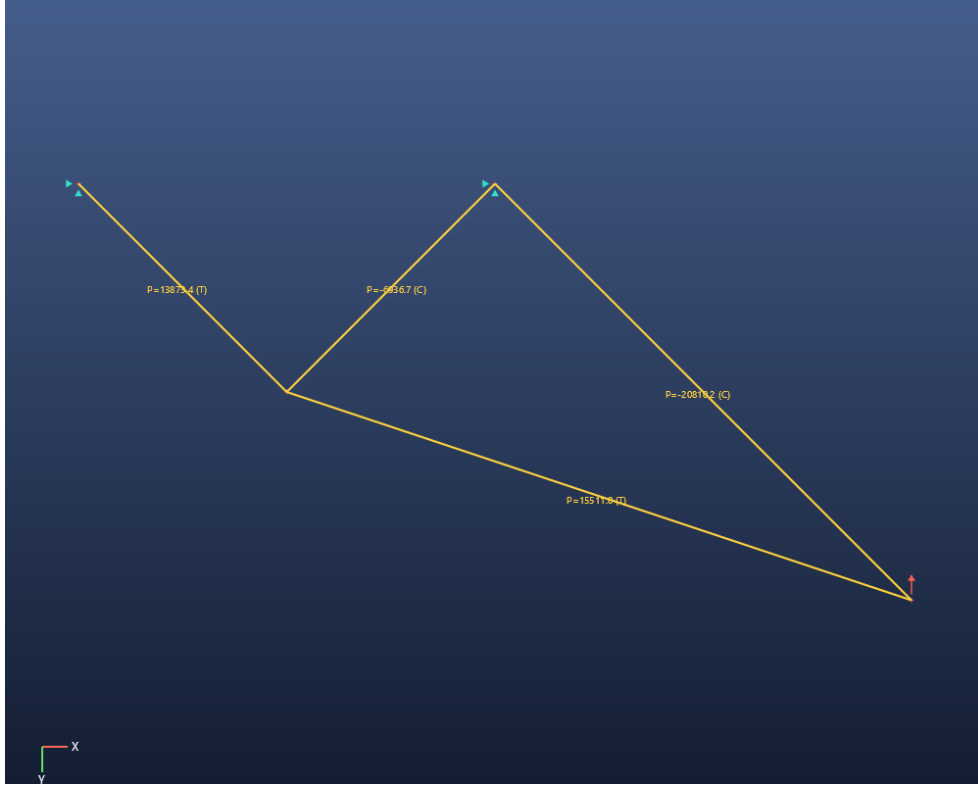
Figure 5.4: E4: SSLL11 articulated truss — pinned supports at A, B (cyan), tip load at D (red), and the solved rod forces (T tension, C compression).
