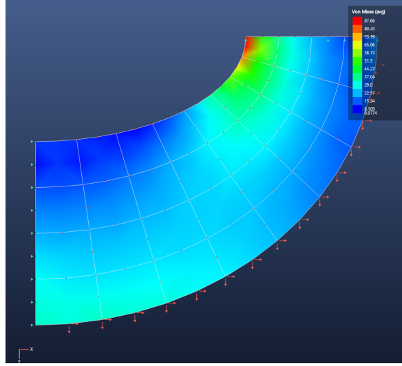
Figure 5.1: E1: LE1 elliptic membrane (fine Quad8 mesh), von Mises field; boundary nodes lie exactly on the ellipses.
