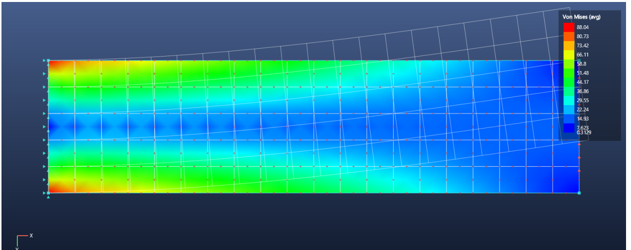
Figure 5.2: E2: SSLP01 deep cantilever under end shear ( 20 \times 5 Quad8), von Mises field with the deformed shape overlaid.
