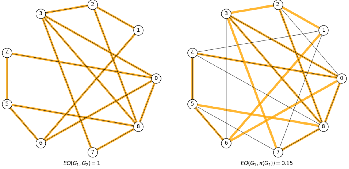
Figure 2.1: Diagram depicting how the choice of vertex mapping affects the edge overlap (EO) between G_1 in orange and G_2 in black. (Left) depicts the case when the two graphs are maximally aligned, (right) depicts the random case with misalignment.
