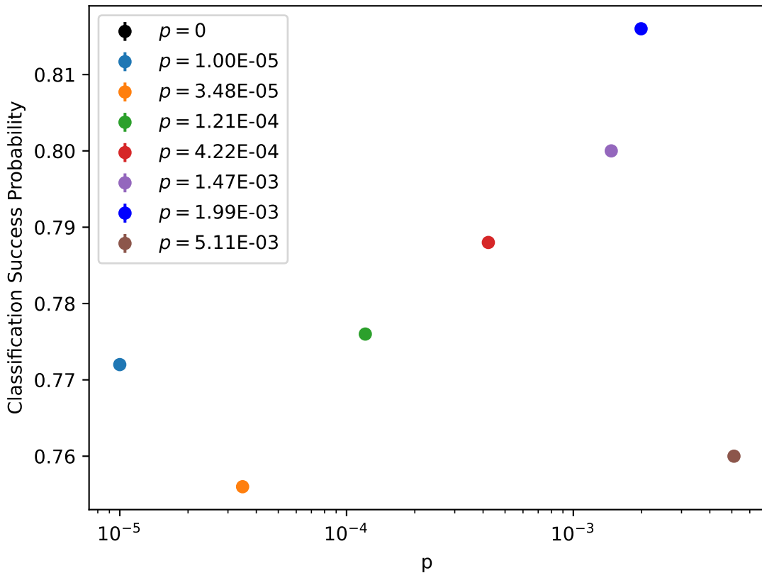
Accuracy vs Depolarising Noise: 20 Layers, 10 Qubits, Noise Model: Single Qubit Depol
