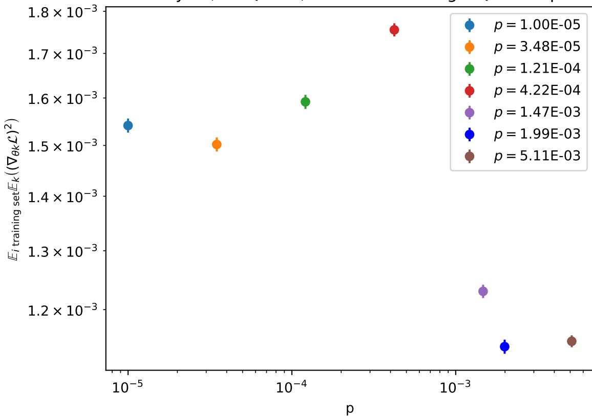
Average Gradient vs Depolarising Noise: 20 Layers, 10 Qubits, Noise Model: Single Qubit Depol
