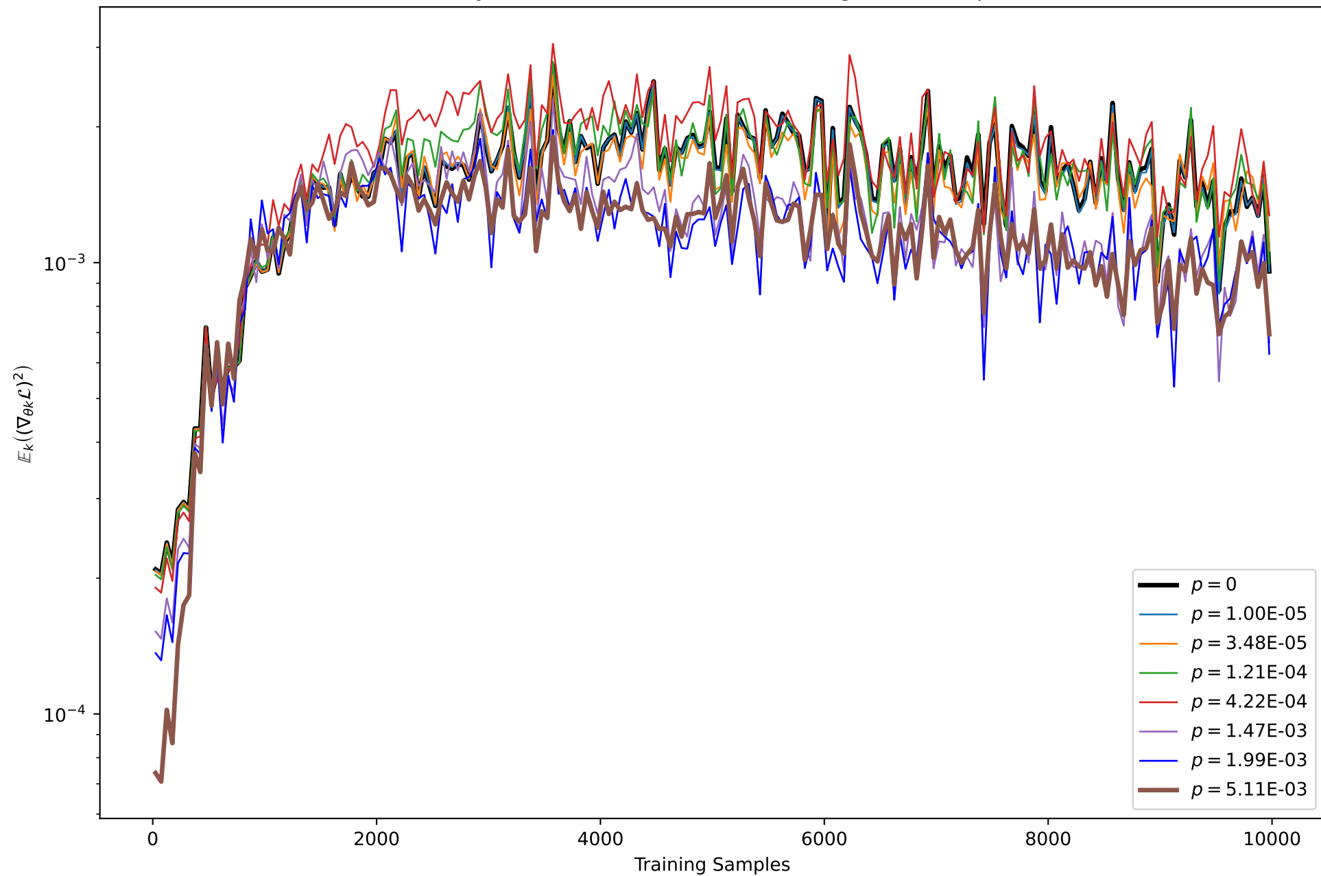
Batch Average Gradients vs Training Samples 20 Layers, 10 Qubits, Noise Model: Single Qubit Depol
