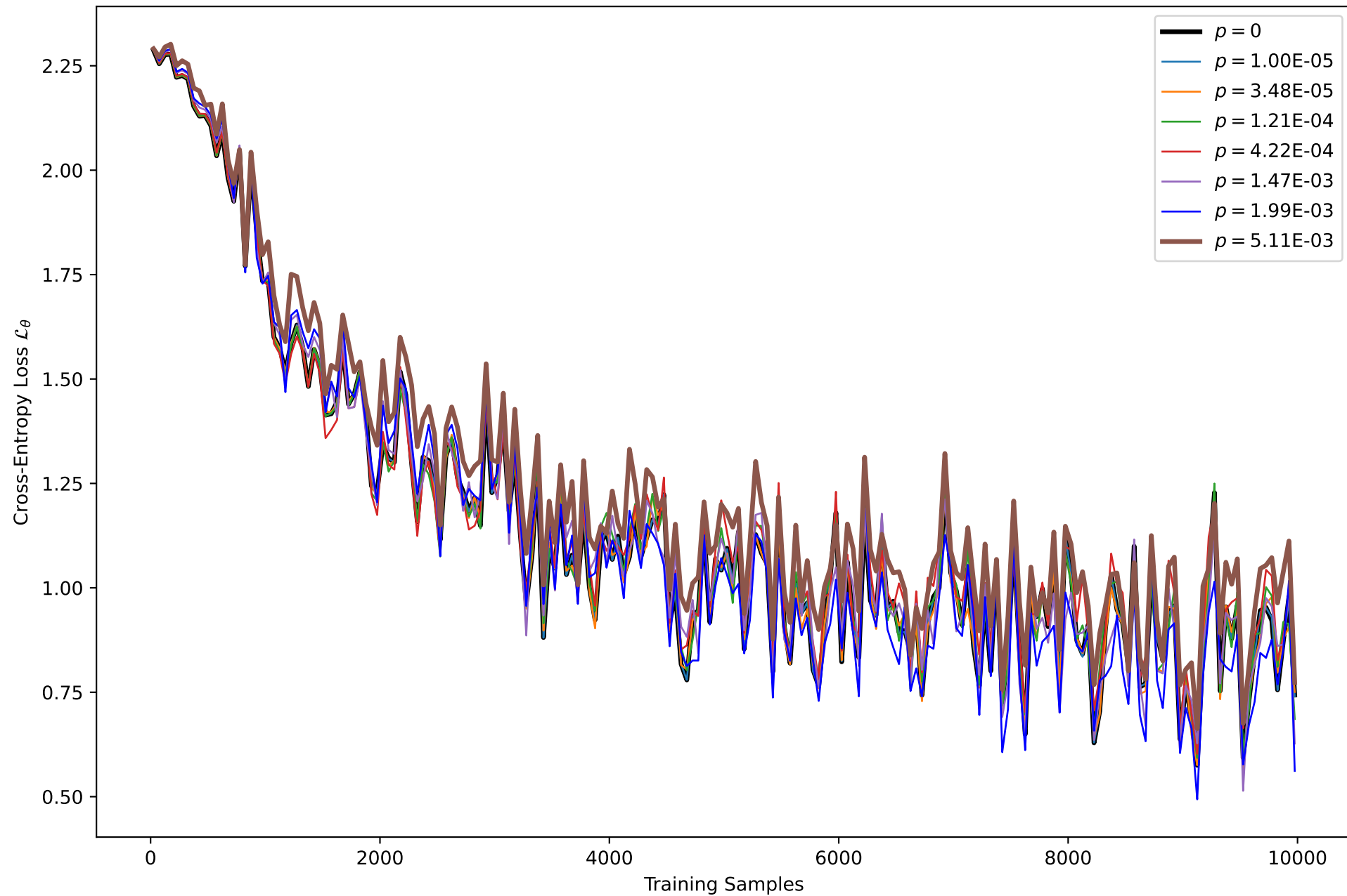
Loss Values vs Training Samples 20 Layers, 10 Qubits, Noise Model: Single Qubit Depol
