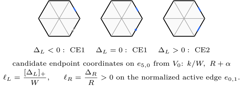
FIGURE 14. The exact sign test for the candidate companion trace, including the CE1 point-contact case.
