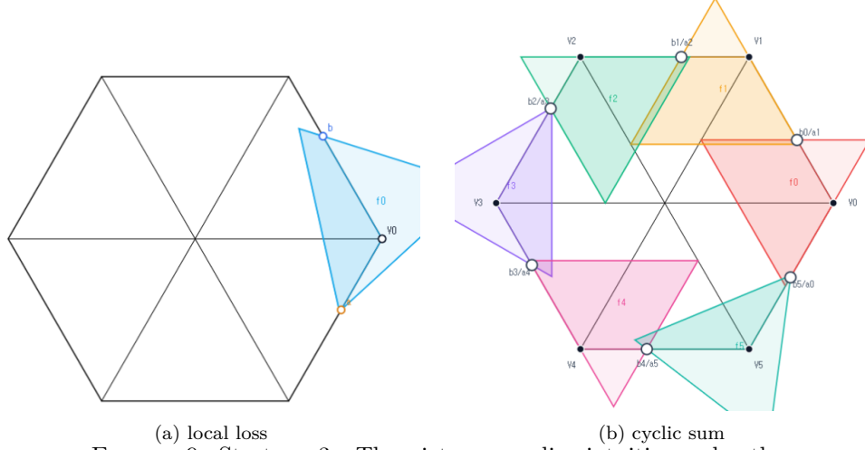
FIGURE 9. Strategy 3. The picture supplies intuition only; the proof uses the three inequalities in Proposition 5.1.
