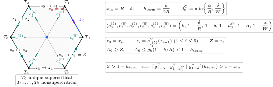
FIGURE 8. The five-V-triangle return mechanism. Geometry supplies the initial demand, five radial parameters, and the terminal cap; the appendix proves the single returned-demand inequality.
