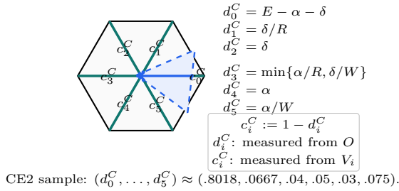
FIGURE 15. The six exact center exits d_i^C and complementary radial demands c_i^C = 1 - d_i^C .
