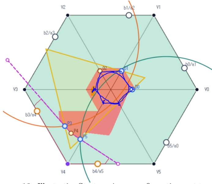
FIGURE 10. Illustrative Strategy 4 core configuration, not to scale. It is an example only; no exclusion, forcing, or enclosure inequality is inferred from the picture.
