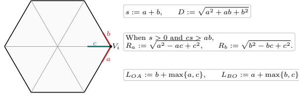
FIGURE 11. The scalar and caliper-denominator data entering the exact admissible-set formula.
