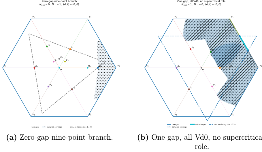
FIGURE 10. Trace-exact AB-envelope snapshots: Zero-gap nine-point branch; One gap, all Vd0, no supercritical role.
