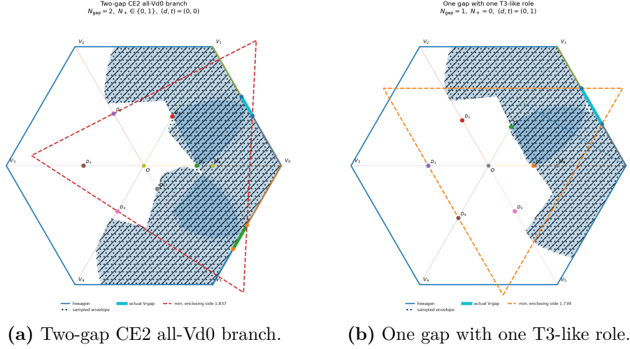
FIGURE 11. Trace-exact AB-envelope snapshots: Two-gap CE2 all-Vd0 branch; One gap with one T3-like role.
