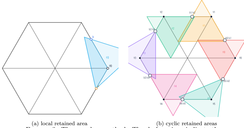
(a) local retained area (b) cyclic retained areas FIGURE 3. The area-loss method. The dark regions indicate the portions retained in H ; the loss \mathcal{L}(T) is the area outside H .
