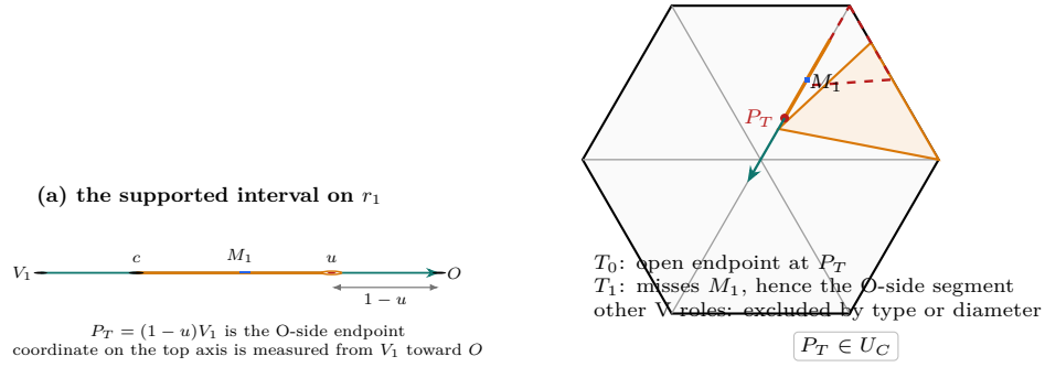
FIGURE 4. Construction of the T3-like rescuer endpoint. The interval [c, u] is parametrized from V_1 toward O , so its O-side endpoint is P_T = (1 - u)V_1 . The T3-like open role omits its endpoint, the adjacent supercritical role contains V_1 but misses M_1 and therefore misses the O-side segment by convexity, and all remaining V roles are excluded. Thus P_T is forced into the C triangle.
