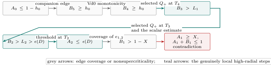
CE1 reverse path: from a deficient terminal to the final contradiction
