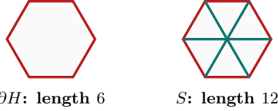
FIGURE 8. The two one-dimensional targets. The full skeleton is used only under the hypotheses of the corresponding trace budget.
