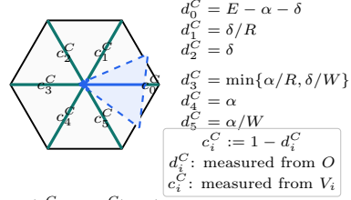
FIGURE 6. The six exact center exits d_i^C and complementary radial reach lower bounds c_i^C = 1 - d_i^C .
