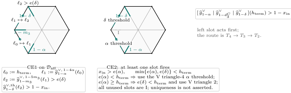
FIGURE 21. The affine slots certified on \mathcal{D}_{\text{aff}} and the two CE2 threshold alternatives. In CE2 at least one threshold fires; uniqueness is not used.
