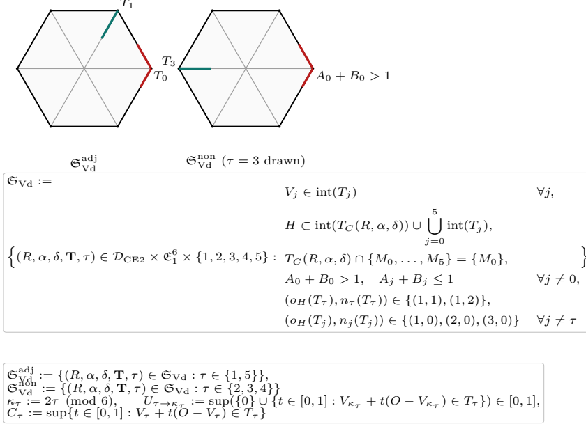
FIGURE 25. The exact CE2 state domain \mathfrak{S}_{\text{Vd}} = \mathfrak{S}_{\text{Vd}}^{\text{adj}} \sqcup \mathfrak{S}_{\text{Vd}}^{\text{non}} for the adjacent and nonadjacent one-Vd residual certificates.
