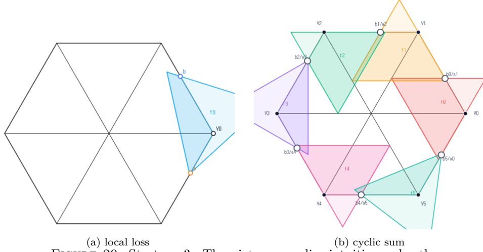
FIGURE 29. Strategy 3. The picture supplies intuition only; the proof uses the three inequalities in Proposition 5.1.
