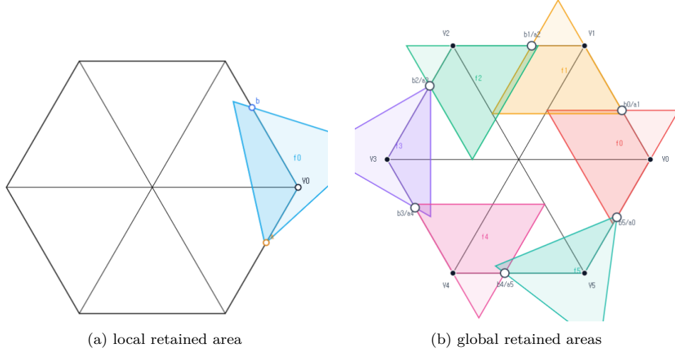
FIGURE 39. Schematic views of Strategy 3, not to scale. The local panel shows one vertex role with boundary reaches a, b , and the global panel shows the six cyclic roles. Only the darker portions represent area retained inside H ; the proof uses the inequalities below, not the picture.
