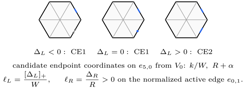
FIGURE 34. The exact sign test for the candidate companion trace, including the CE1 point-contact case.
