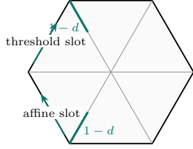
FIGURE 18. The general affine and threshold decorated maps, with their certification domains, on retained Strategy 2 skeleton V triangles.
