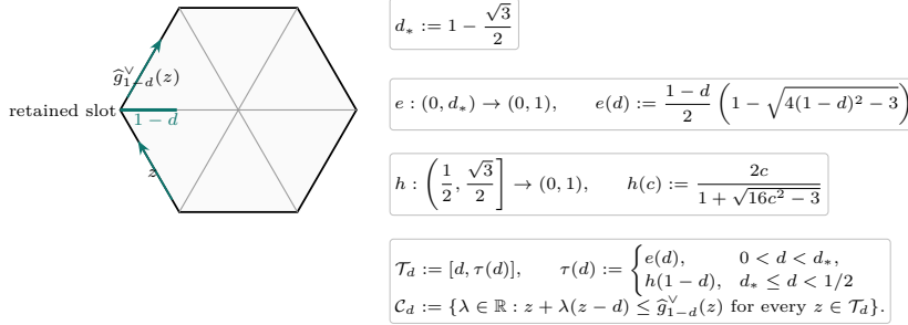
FIGURE 17. The exact domains d_* , e , h , \mathcal{T}_d , \tau , and \mathcal{C}_d for the decorated lower relaxations.
