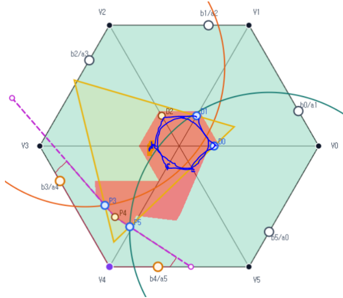
FIGURE 30. Illustrative Strategy 4 core configuration, not to scale. It is an example only; no exclusion, forcing, or enclosure inequality is inferred from the picture.
