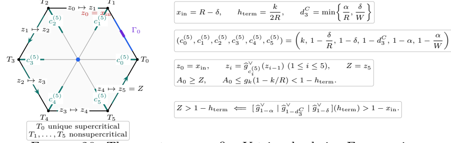
FIGURE 20. The exact one-gap five-V-triangle chain. Every z_j is a formal lower bound for the incoming reach at the corresponding skeleton V triangle.
