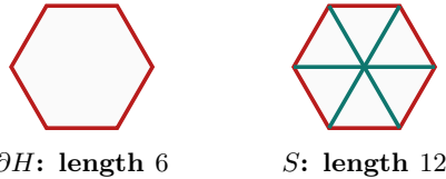
FIGURE 11. The perimeter and the conditional full-skeleton target. The proof uses only the numerical trace caps stated below.
