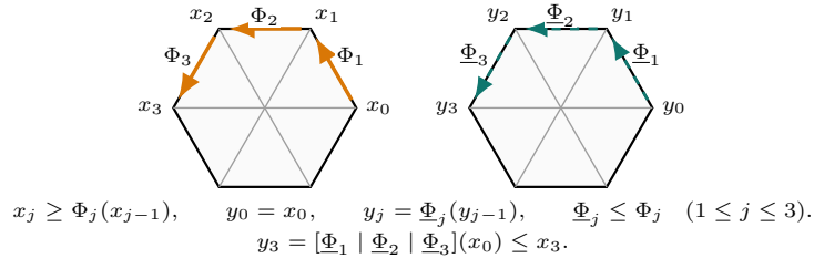
FIGURE 12. Exact and lower-relaxed states on consecutive hexagon-skeleton V triangles. The internal edges used by an identity relaxation are center-free; endpoint center intervals are first absorbed into residual demands.
