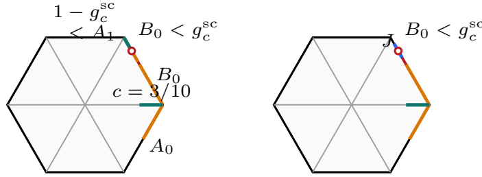
U_C \cap e_{0,1} = \emptyset \quad J \neq \emptyset : \quad B_0 < g_c^{sc} \not\approx A_1 > 1 - g_c^{sc} FIGURE 7. A representative strict-supercritical envelope configuration. Its outgoing bound is unconditional; only a center-free edge permits the complementary next-V-triangle bound.
