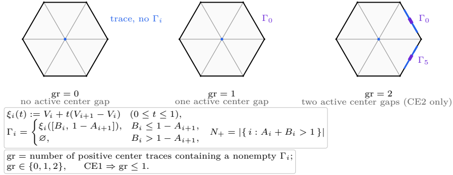
FIGURE 15. The three active-gap ranks. A singleton \Gamma_i remains a nonempty V -gap and is counted.
