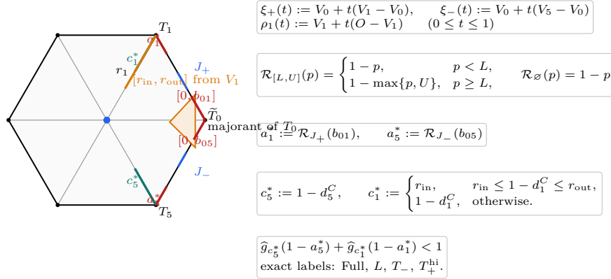
FIGURE 23. The support-isolated T3-like V triangle, its two center-assisted boundary residuals, and its two forced endpoint radial demands.
