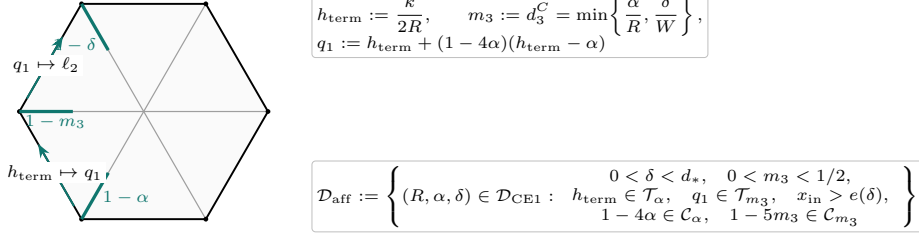
FIGURE 19. The certified CE1 double-selected- T_+ subdomain \mathcal{D}_{\text{aff}} and its two retained affine states.
