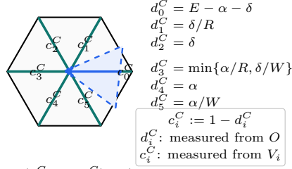
FIGURE 35. The six exact center exits d_i^C and complementary radial demands c_i^C = 1 - d_i^C .
