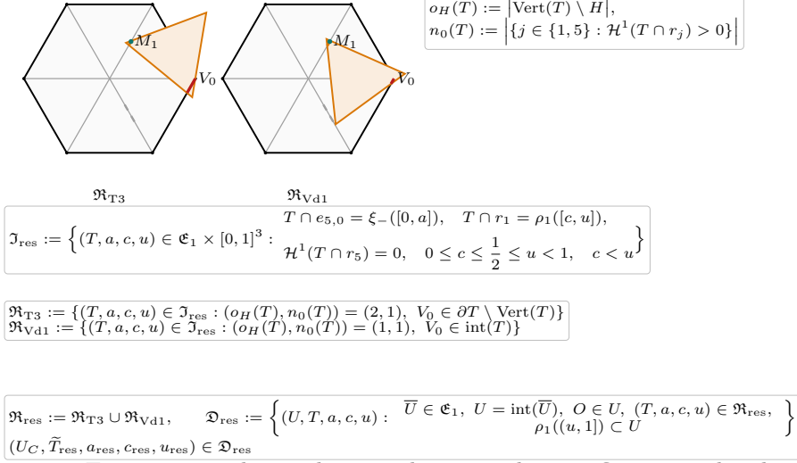
FIGURE 24. The mathematical rescuer domain \mathfrak{D}_{res} : translated T3-like majorants and adjacent Vd1 closures enter one exact tuple interface.
