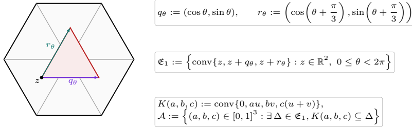
FIGURE 3. The oriented unit-triangle family \mathfrak{E}_1 and the formal containment definition of the local admissible set \mathcal{A} .
