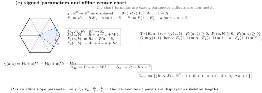
FIGURE 33. The affine center chart and the exact dependency structure of the signed parameters.
