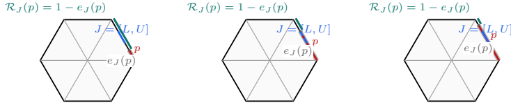
FIGURE 6. The three geometric cases in the residual operator \mathcal{R}_{[L, U]}(p) , drawn on a handoff edge.
