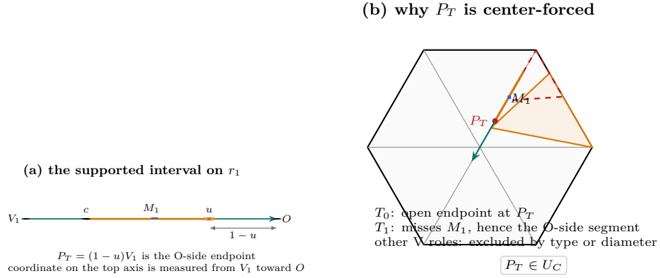
FIGURE 14. Construction of the T3-like rescuer endpoint. The interval [c, u] is parametrized from V_1 toward O , so its O-side endpoint is P_T = (1 - u)V_1 . The T3-like open role omits its endpoint, the adjacent supercritical role contains V_1 but misses M_1 and therefore misses the O-side segment by convexity, and all remaining V roles are excluded. Thus P_T is forced into the C triangle.
