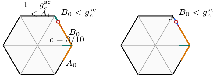
U_C \cap e_{0,1} = \emptyset \quad J \neq \emptyset : B_0 < g_c^{sc} \not\Rightarrow A_1 > 1 - g_c^{sc} FIGURE 9. A representative strict-supercritical envelope configuration. Its outgoing bound is unconditional; only a center-free edge permits the complementary next-V-triangle bound.
