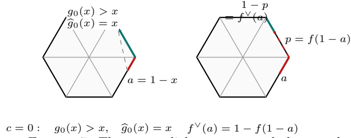
FIGURE 7. The zero-radial geometry and the complement dual. The identity is \hat{g}_0 , not raw g_0 .
