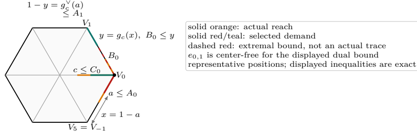
FIGURE 6. Selected demands, actual V-triangle reaches, incoming defect, raw extremal output, and the center-free complementary handoff.
