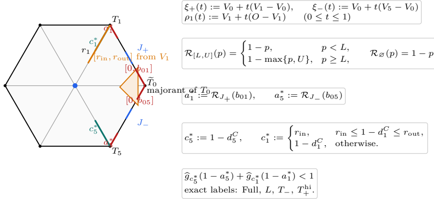
FIGURE 25. The support-isolated T3-like V triangle, its two center-assisted boundary residuals, and its two forced endpoint radial demands.
