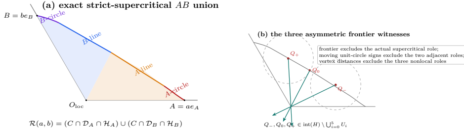
FIGURE 6. The strict-supercritical AB frontier and the three asymmetric witnesses. The source-conditioned union has, in counterclockwise order, an A -circle arc, an A -line segment, a B -line segment, and a B -circle arc. The points Q_-, Q_0, Q_+ are selected on this exact frontier and are then excluded from the six actual V roles by frontier, moving-circle, and vertex-distance arguments. The drawing is schematic; the labelled frontier order and witness roles are exact.
