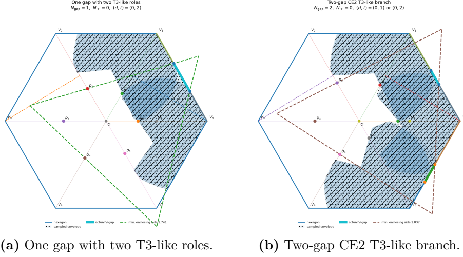
FIGURE 19. Trace-exact AB-envelope snapshots: One gap with two T3-like roles; Two-gap CE2 T3-like branch.
