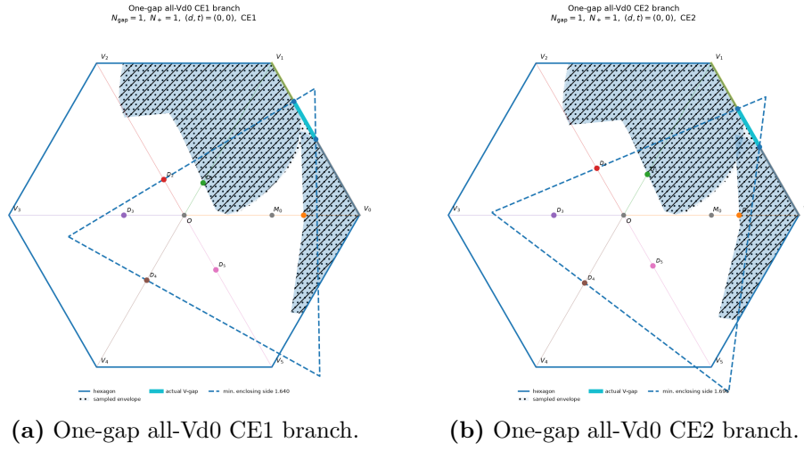
FIGURE 20. Trace-exact AB-envelope snapshots: One-gap all-Vd0 CE1 branch; One-gap all-Vd0 CE2 branch.
