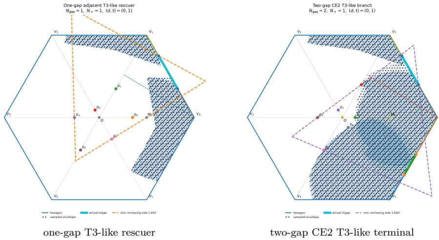
FIGURE 14. The two gap-rank outputs of the exactly-one-T3-like row.
