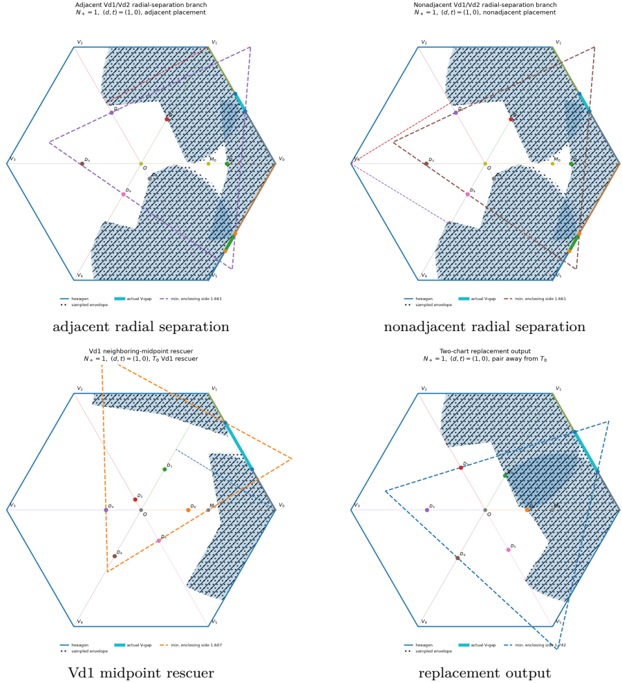
FIGURE 15. The four one-Vd placement outputs, now stated as separate propositions rather than hidden in one proof.
