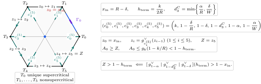
FIGURE 8. The five-V-triangle return mechanism. Geometry supplies the initial demand, five radial parameters, and the terminal cap; the appendix proves the single returned-demand inequality.
