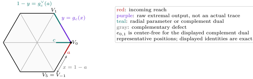
FIGURE 6. Incoming reach and defect, radial parameter, raw extremal output, and the center-free lower transfer.
