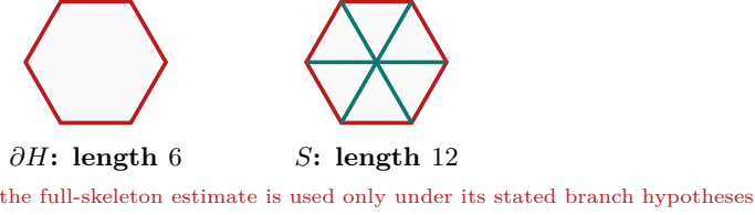
FIGURE 13. The two one-dimensional targets. The full skeleton is used only under the hypotheses of the corresponding trace budget.
