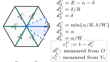
FIGURE 11. The six exact center exits d_i^C and complementary radial lower bounds c_i^C = 1 - d_i^C .
