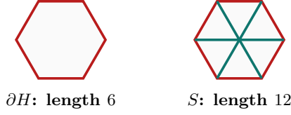
FIGURE 3. The perimeter and the full skeleton. The skeleton is used only under the hypotheses of the corresponding trace bound.
