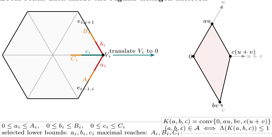
FIGURE 2. The three maximal reaches, selected lower bounds, and the associated anchor hull. The least equilateral enclosure side of this hull controls both boundary propagation and the nine-point obstruction.
