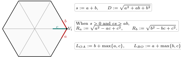
FIGURE 7. The scalar and caliper-denominator data entering the exact admissible-set formula.
