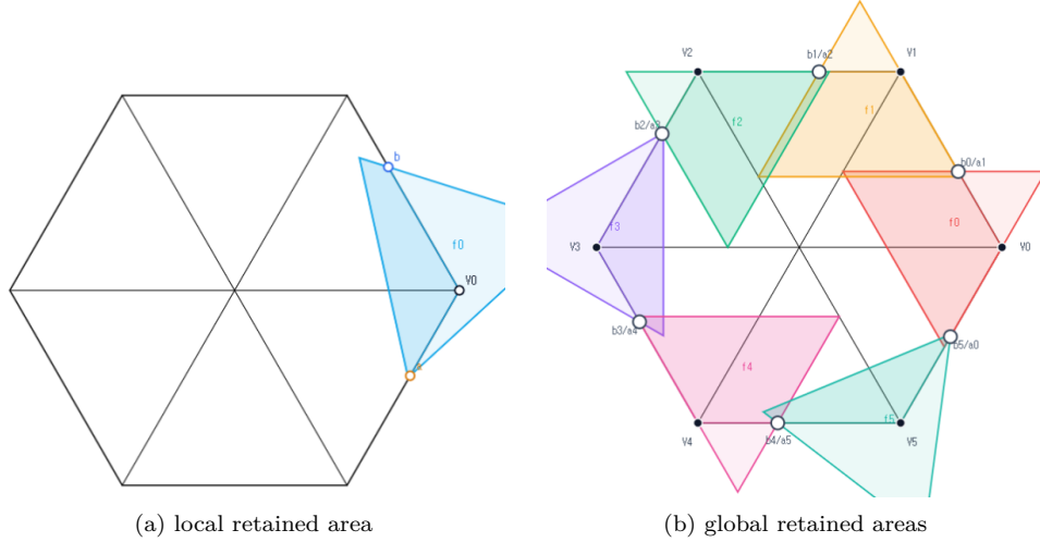
FIGURE 15. Schematic views of Method 3, not to scale. The local panel shows one vertex triangle with boundary reaches a, b , and the global panel shows the six cyclic triangles. Only the darker portions represent area retained inside H ; the proof uses the inequalities below, not the picture.
