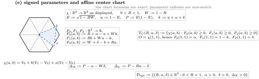
FIGURE 9. The affine center chart and the exact dependency structure of the signed parameters.
