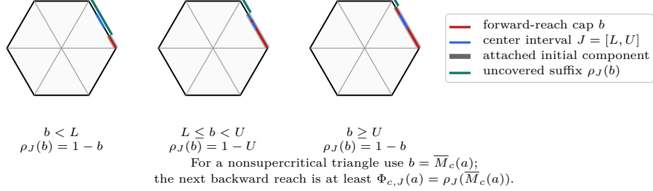
FIGURE 5. The three cases in the uncovered-suffix function \rho_{[L,U]}(b) .
