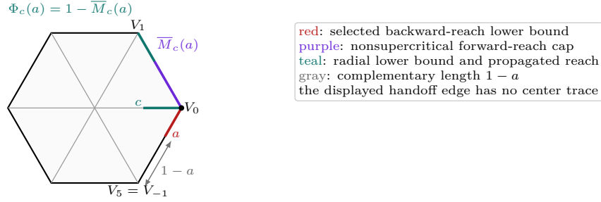
FIGURE 4. Backward reach, radial reach, the maximal forward reach M_c(a) , and the propagated lower bound \Phi_c(a) .
