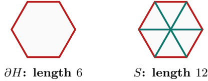
FIGURE 4. The perimeter and full-skeleton targets. The skeleton is used only under the hypotheses of the corresponding trace budget.
