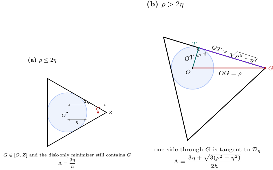
FIGURE 12. The two minimizing configurations in the disk-plus-point formula. For \rho \leq 2\eta , the centered equilateral triangle tangent to \mathcal{D}_\eta already contains G . For \rho > 2\eta , the point G becomes a vertex of the minimizing triangle and one incident side is tangent to the disk. The tangent length GT = \sqrt{\rho^2 - \eta^2} is the geometric source of the radical term.
