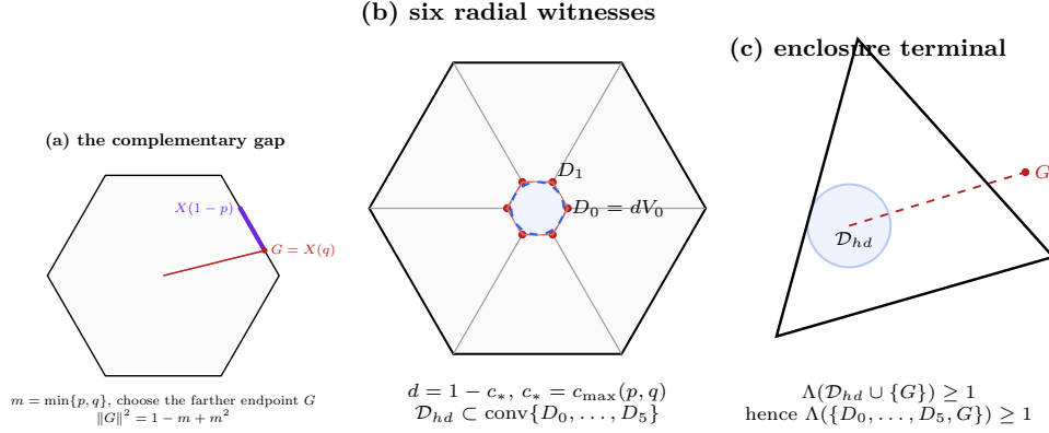
FIGURE 6. The complementary-gap enclosure mechanism. The farther endpoint G of J(p, q) is center-forced. Common-pair domination produces the six center-forced points D_i = (1 - c_*)V_i , whose convex hull contains the disk \mathcal{D}_{h(1-c_*)} . The disk-plus-point formula then forces enclosing side length at least one. The disk is not an additional witness; it is contained in the convex hull of the six finite radial witnesses.
