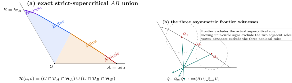
FIGURE 14. The strict-supercritical AB frontier and the three asymmetric witnesses. The source-conditioned union has, in counterclockwise order, an A -circle arc, an A -line segment, a B -line segment, and a B -circle arc. The points Q_-, Q_0, Q_+ are selected on this exact frontier and are then excluded from the six actual V roles by frontier, moving-circle, and vertex-distance arguments. The drawing is schematic; the labelled frontier order and witness roles are exact.
