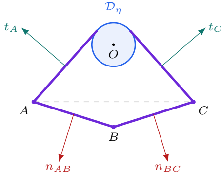
FIGURE 15. The four-contact terminal for the zero-gap witness. The supporting lines through AB and BC and the two outer disk tangencies exhaust the active changes of support source. The dashed segment AC is not exposed: B and the disk center lie on opposite sides. The drawing is schematic; the exact witness geometry and the paired tangent residuals are proved in the text. No auxiliary Minkowski sum or cap covering is needed.
