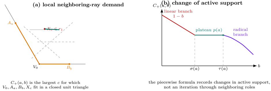
FIGURE 11. Geometry behind the neighboring-ray capacity C_+(a, b) . The local problem asks how far a triangle anchored at V_0 and the two boundary points A_a, B_b can reach on the neighboring arm r_1 . As b varies with a fixed, the active support pattern changes from the linear branch to a plateau and then to the radical branch, with transition points \sigma(a) and \tau(a) . The graph is schematic; the transition order, endpoint selection, and branch labels are exact.
