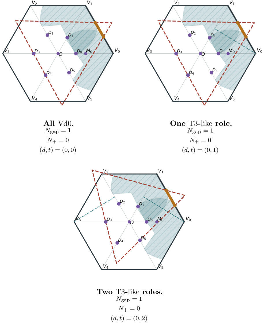
FIGURE 7. Case A: sampled complementary-gap data.
