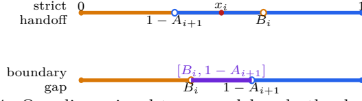
FIGURE 4. One-dimensional trace model; only the drawn lengths are schematic. The top panel shows a strict handoff in the overlap (1 - A_{i+1}, B_i) . The bottom panel shows the closed gap [B_i, 1 - A_{i+1}] ; when its endpoints coincide, the resulting singleton is still uncovered by the two open traces.
