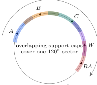
FIGURE 11. Schematic support-cap chain, not to scale. The drawing explains the cyclic covering mechanism only. The overlap inequalities are proved in Appendices E and G.
