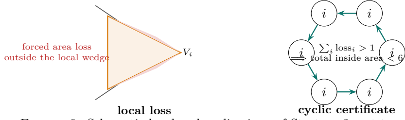
FIGURE 9. Schematic local and cyclic views of Strategy 3, not to scale. The shaded regions suggest the forced exterior loss; the exact inequalities are proved independently in Appendix D.
