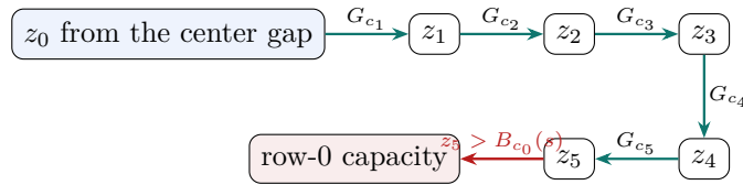
FIGURE 6. Schematic five-row propagation for a one-gap branch.
