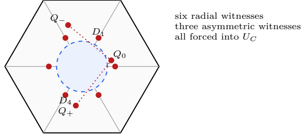
FIGURE 10. Schematic Strategy 4 witness, not to scale. The six radial points are symbolically exact; the locations of Q_-, Q_0, Q_+ vary with (a, b) . No exclusion or enclosure inequality is inferred from the picture.
