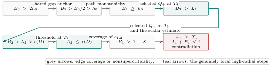
FIGURE 8. Logical structure of the CE1 direct reverse-path certificate. The proof starts from the BC tail input (with h_0 = Q ), moves through the actual boundary reaches, uses two selected-arc estimates and one high-radial threshold, and returns to T_1 with incompatible incoming and outgoing demands.
