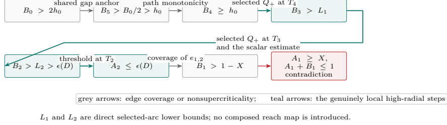
FIGURE 8. Logical structure of the CE1 direct reverse-path certificate. The proof starts from the BC tail input (with h_0 = Q ), moves through the actual boundary reaches, uses two selected-arc estimates and one high-radial threshold, and returns to T_1 with incompatible incoming and outgoing demands.
