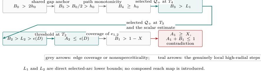
FIGURE 6. Logical structure of the CE1 direct reverse-path certificate. The proof starts from the BC tail input, moves through the actual boundary reaches, uses two selected-arc estimates and one high-radial threshold, and returns to T_1 with incompatible incoming and outgoing demands.
