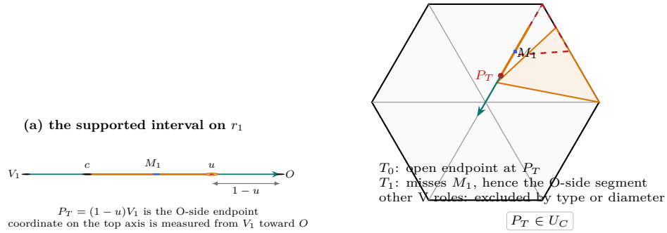
FIGURE 7. Construction of the T3-like rescuer endpoint. The interval [c, u] is parametrized from V_1 toward O , so its O-side endpoint is P_T = (1 - u)V_1 . The T3-like open role omits its endpoint, the adjacent supercritical role contains V_1 but misses M_1 and therefore misses the O-side segment by convexity, and all remaining V roles are excluded. Thus P_T is forced into the C triangle.
