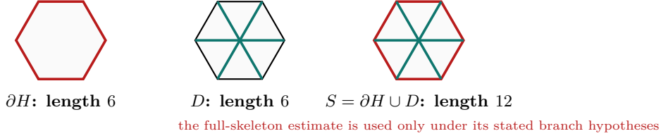
FIGURE 4. Exact targets and their one-dimensional measures. The coloring is explanatory. The full-skeleton panel is conditional, not a claim that seven unit triangles can never cover S .
