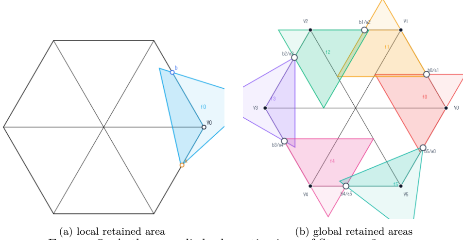
FIGURE 5. Author-supplied schematic views of Strategy 3, not to scale. The local panel shows one vertex-role triangle with boundary reaches a, b , and the global panel shows the six cyclic vertex-role triangles. Only the darker colored portions represent area retained inside H . The exact loss inequalities and cyclic sums are proved independently in Section 5.
