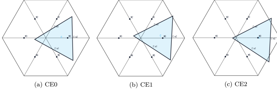
(a) CE0 (b) CE1 (c) CE2 FIGURE 2. Illustrative examples of the three center-role types. The screenshots are not to scale, and no proof depends on visual inspection.
