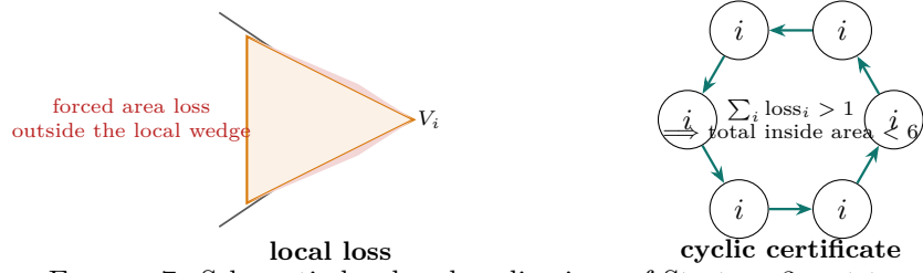
FIGURE 7. Schematic local and cyclic views of Strategy 3, not to scale. The shaded regions suggest the forced exterior loss; the exact inequalities are proved independently in Appendix D.
