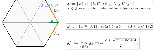
FIGURE 8. The interval family \mathfrak{J} , strict-supercritical input set, and its supremal output, shown on the skeleton.
