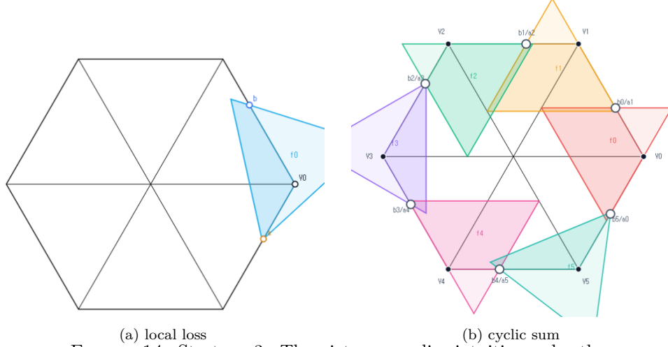
FIGURE 14. Strategy 3. The picture supplies intuition only; the proof uses the three inequalities in Proposition 5.1.
