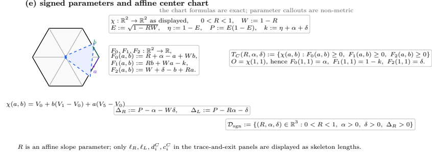
FIGURE 18. The affine center chart and the exact dependency structure of the signed parameters.
