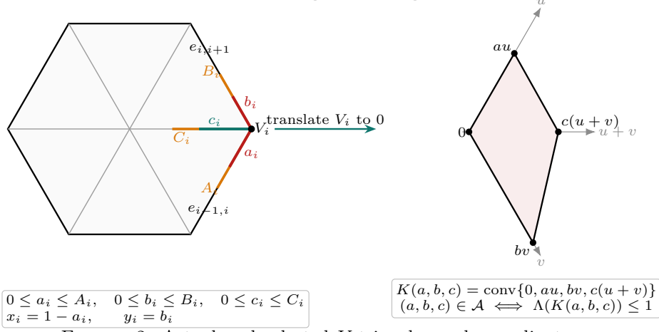
FIGURE 2. Actual and selected V-triangle reach coordinates on the full hexagon skeleton, together with the rigid local demand hull. The least equilateral enclosure side of that hull is the scalar controlling both Strategy 2 transfers and Strategy 4 witnesses.
