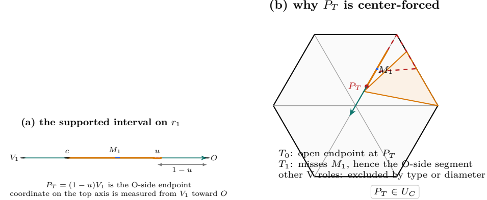
FIGURE 6. Construction of the T3-like rescuer endpoint. The interval [c, u] is parametrized from V_1 toward O , so its O-side endpoint is P_T = (1 - u)V_1 . The T3-like open role omits its endpoint, the adjacent supercritical role contains V_1 but misses M_1 and therefore misses the O-side segment by convexity, and all remaining V roles are excluded. Thus P_T is forced into the C triangle.
