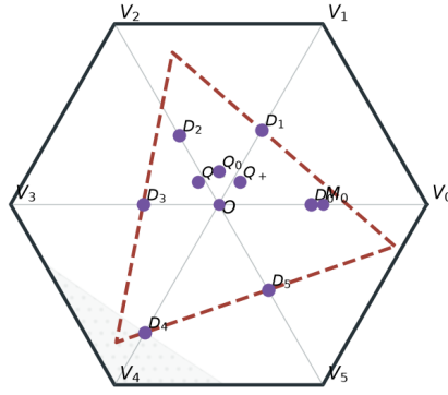
Trace-exact witness.
