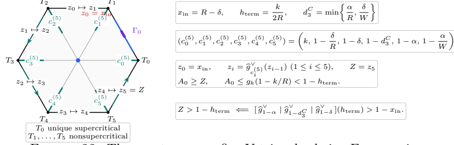
FIGURE 22. The exact one-gap five-V-triangle chain. Every z_j is a formal lower bound for the incoming reach at the corresponding skeleton V triangle.
