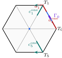
one active gap
