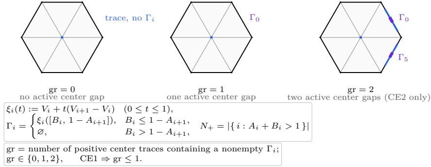
FIGURE 17. The three active-gap ranks. A singleton \Gamma_i remains a nonempty V-gap and is counted.
