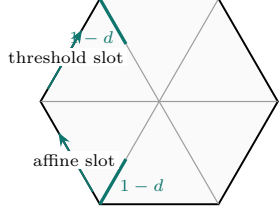
FIGURE 20. The general affine and threshold decorated maps, with their certification domains, on retained Strategy 2 skeleton V triangles.
