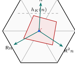
FIGURE 5. The support-function definition of the equilateral enclosure gauge, placed in the full skeleton containing the local demand hull. This figure is a geometric sketch; the exact caliper equations are in Appendix D.
