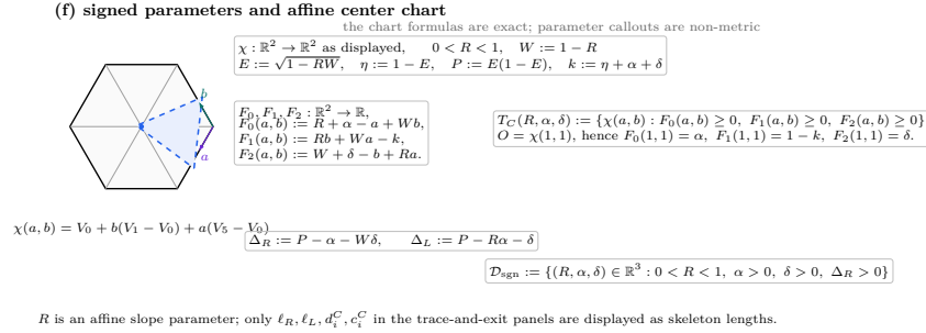
FIGURE 35. The affine center chart and the exact dependency structure of the signed parameters.
