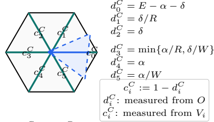
FIGURE 37. The six exact center exits d_i^C and complementary radial demands c_i^C = 1 - d_i^C .
