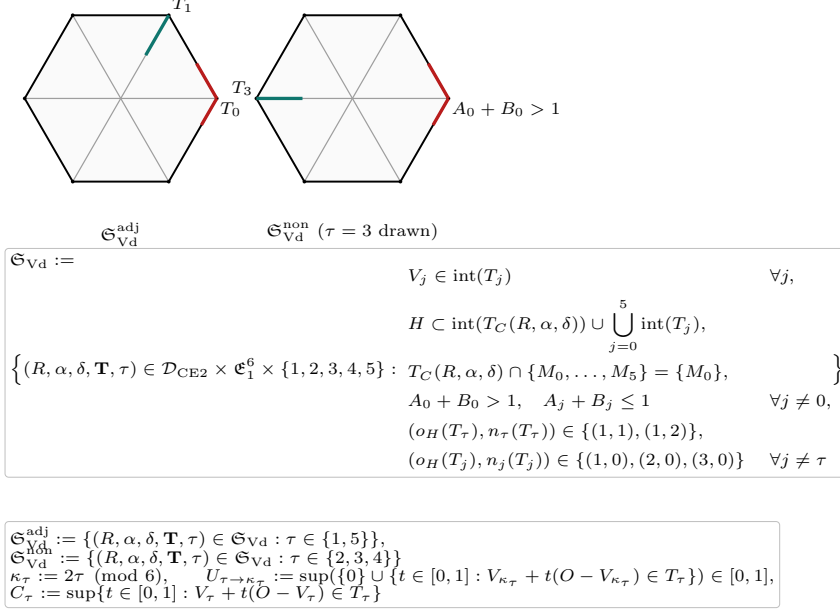
FIGURE 27. The exact CE2 state domain \mathfrak{S}_{\text{Vd}} = \mathfrak{S}_{\text{Vd}}^{\text{adj}} \sqcup \mathfrak{S}_{\text{Vd}}^{\text{non}} for the adjacent and nonadjacent one-Vd residual certificates.
