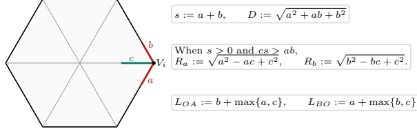
FIGURE 33. The scalar and caliper-denominator data entering the exact admissible-set formula.
