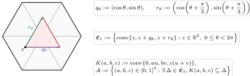
FIGURE 4. The oriented unit-triangle family \mathfrak{E}_1 and the formal containment definition of the local admissible set \mathcal{A} .
