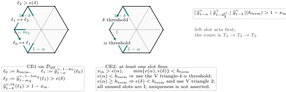
FIGURE 23. The affine slots certified on \mathcal{D}_{\text{aff}} and the two CE2 threshold alternatives. In CE2 at least one threshold fires; uniqueness is not used.
