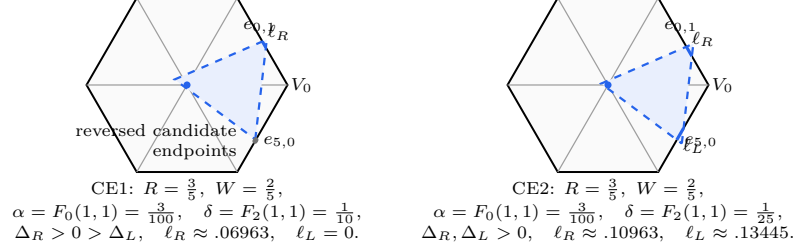
FIGURE 12. Representative CE1 and CE2 center triangles on the full skeleton. The blue segments are the geometric boundary traces; exact parameter equations are in Appendix E.
