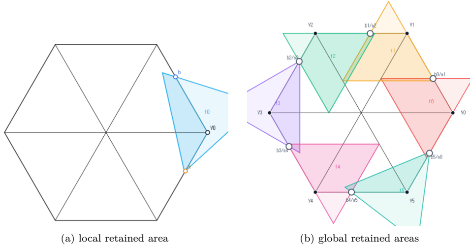
FIGURE 41. Schematic views of Strategy 3, not to scale. The local panel shows one vertex role with boundary reaches a, b , and the global panel shows the six cyclic roles. Only the darker portions represent area retained inside H ; the proof uses the inequalities below, not the picture.
