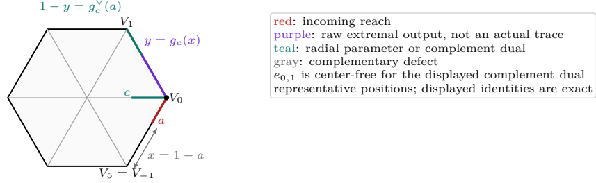
FIGURE 6. Incoming reach and defect, radial parameter, raw extremal output, and the center-free complement dual.
