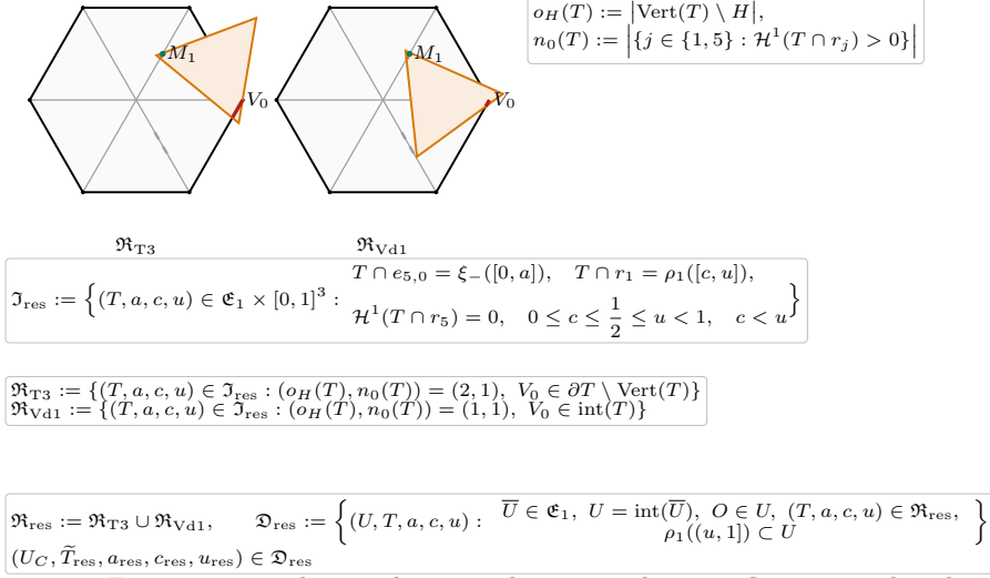
FIGURE 26. The mathematical rescuer domain \mathfrak{D}_{\text{res}} : translated T3-like majorants and adjacent Vd1 closures enter one exact tuple interface.
