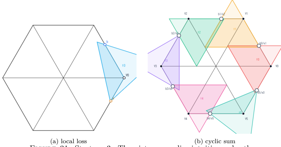
(a) local loss (b) cyclic sum FIGURE 31. Strategy 3. The picture supplies intuition only; the proof uses the three inequalities in Proposition 5.1.
