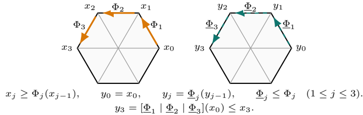
FIGURE 11. Exact and lower-relaxed iterates placed on successive V triangles.
