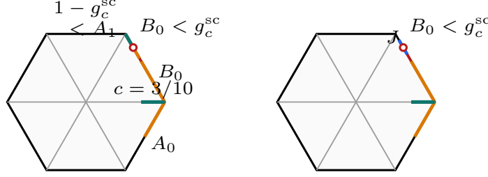
U_C \cap e_{0,1} = \emptyset \quad J \neq \emptyset : \quad B_0 < g_c^{\text{sc}} \not\Rightarrow A_1 > 1 - g_c^{\text{sc}} FIGURE 9. A representative strict-supercritical envelope configuration. Its outgoing bound is unconditional; only a center-free edge permits the complementary next-V-triangle bound.
