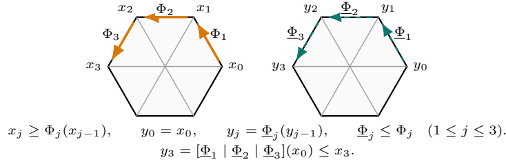
FIGURE 14. Exact and lower-relaxed states on consecutive hexagon-skeleton V triangles. The internal edges used by an identity relaxation are center-free; endpoint center intervals are first absorbed into residual demands.
