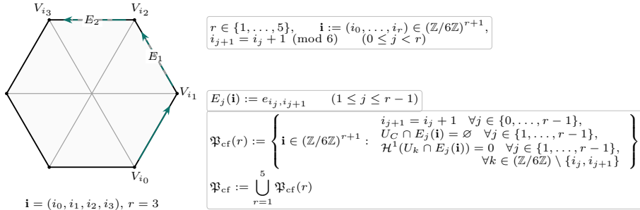
FIGURE 16. A representative element of \mathfrak{P}_{\text{cf}}(3) , including every internal-edge exclusion in the exact center-free ordinary-path set.
