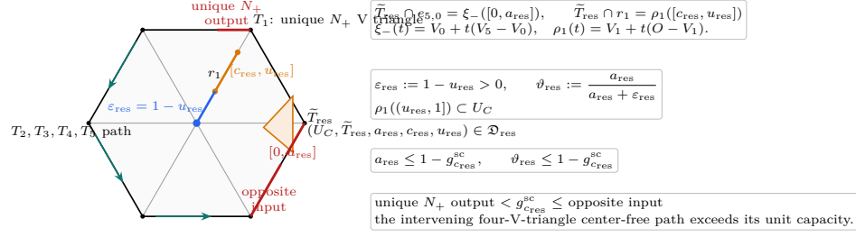
FIGURE 28. The common adjacent-rescuer interface for a T3-like or Vd1 role and the unique strict-supercritical V triangle.
