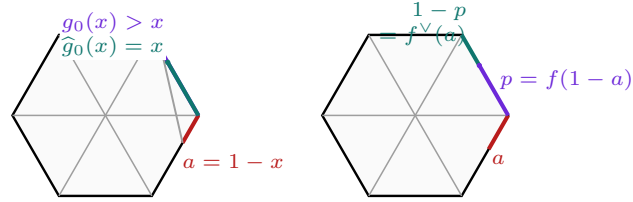
FIGURE 7. The zero-radial geometry and the complement dual. The identity is \widehat{g}_0 , not raw g_0 .
