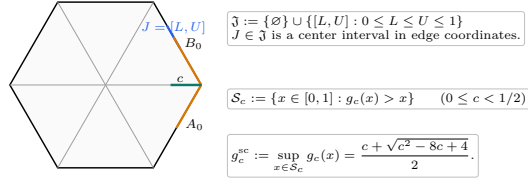
FIGURE 10. The interval family \mathfrak{J} , strict-supercritical input set, and its supremal output, shown on the skeleton.
