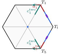
two active gaps; CE2
