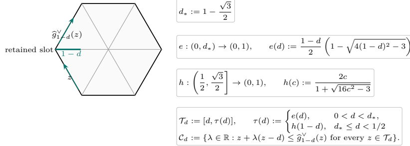
FIGURE 19. The exact domains d_* , e , h , \mathcal{T}_d , \tau , and \mathcal{C}_d for the decorated lower relaxations.
