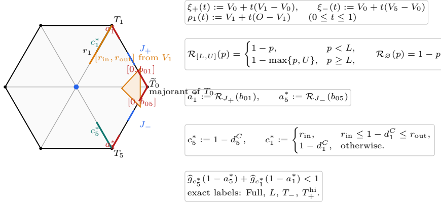
FIGURE 25. The support-isolated T3-like V triangle, its two center-assisted boundary residuals, and its two forced endpoint radial demands.
