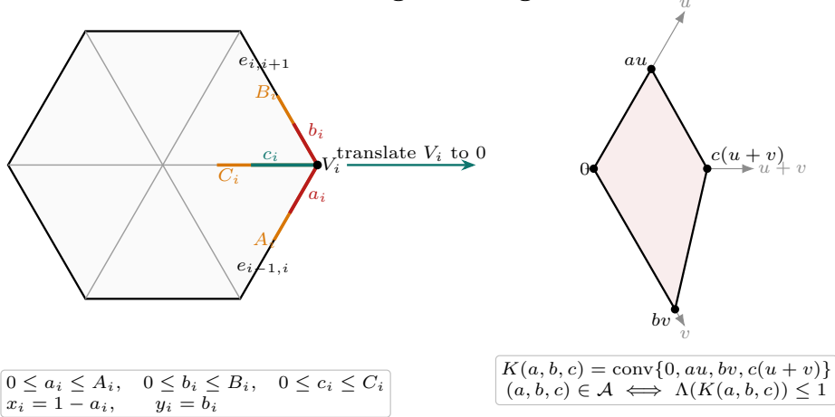
FIGURE 3. Actual and selected V-triangle reach coordinates on the full hexagon skeleton, together with the rigid local demand hull. The least equilateral enclosure side of that hull is the scalar controlling both Strategy 2 transfers and Strategy 4 witnesses.
