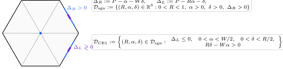
FIGURE 15. The signed parameter domain and its exact CE1/CE2 Strategy 2 subdomains on the two possible center-trace edges.
