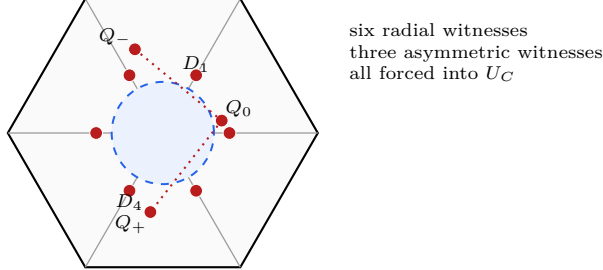
FIGURE 8. Schematic Strategy 4 witness, not to scale. The six radial points are symbolically exact; the locations of Q_-, Q_0, Q_+ vary with (a, b) . No exclusion or enclosure inequality is inferred from the picture.
