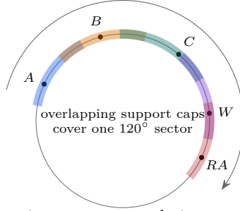
FIGURE 9. Schematic support-cap chain, not to scale. The drawing explains the cyclic covering mechanism only. The overlap inequalities are proved in Appendices E and G.
