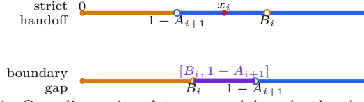
FIGURE 4. One-dimensional trace model; only the drawn lengths are schematic. The top panel shows a strict handoff in the overlap (1 - A_{i+1}, B_i) . The bottom panel shows the closed gap [B_i, 1 - A_{i+1}] ; when its endpoints coincide, the resulting singleton is still uncovered by the two open traces.
