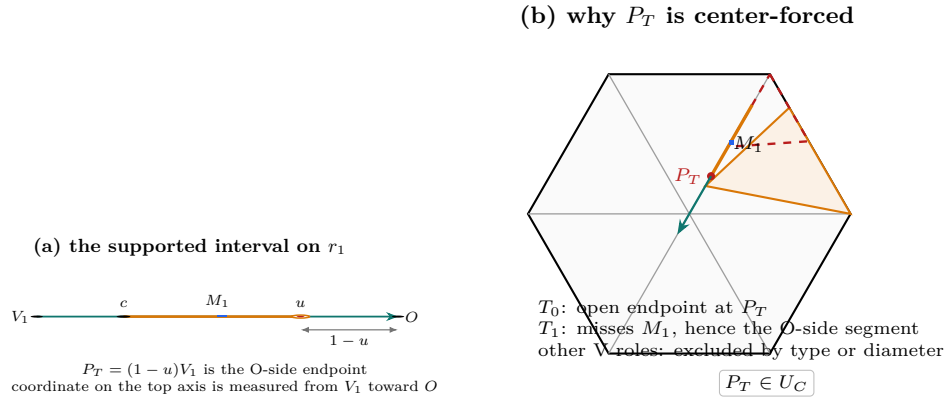
FIGURE 6. Construction of the T3-like rescuer endpoint. The interval [c, u] is parametrized from V_1 toward O , so its O-side endpoint is P_T = (1 - u)V_1 . The T3-like open role omits its endpoint, the adjacent supercritical role contains V_1 but misses M_1 and therefore misses the O-side segment by convexity, and all remaining V roles are excluded. Thus P_T is forced into the C triangle.
