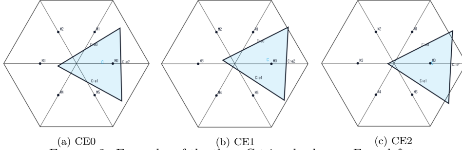
FIGURE 2. Examples of the three C triangle classes. From left to right, the C triangle has positive-length trace on zero, one, and two edges of \partial H ; point contacts do not count. The panels illustrate the classification.
