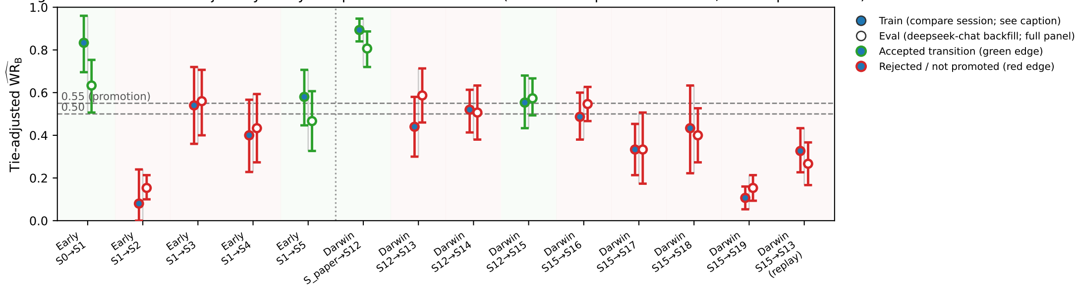
Figure 1b — Extended trajectory: early S0 spine + Darwin reboot (train vs deepseek-chat blind; 95% topic-block CI)
