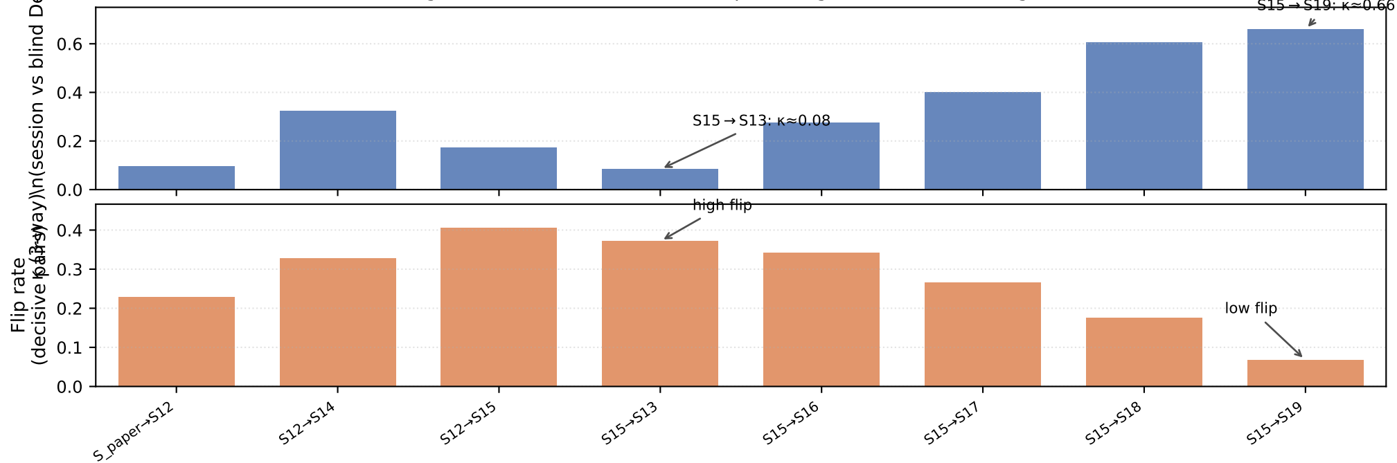
Figure 2 — Session vs blind DeepSeek agreement (chronological)
